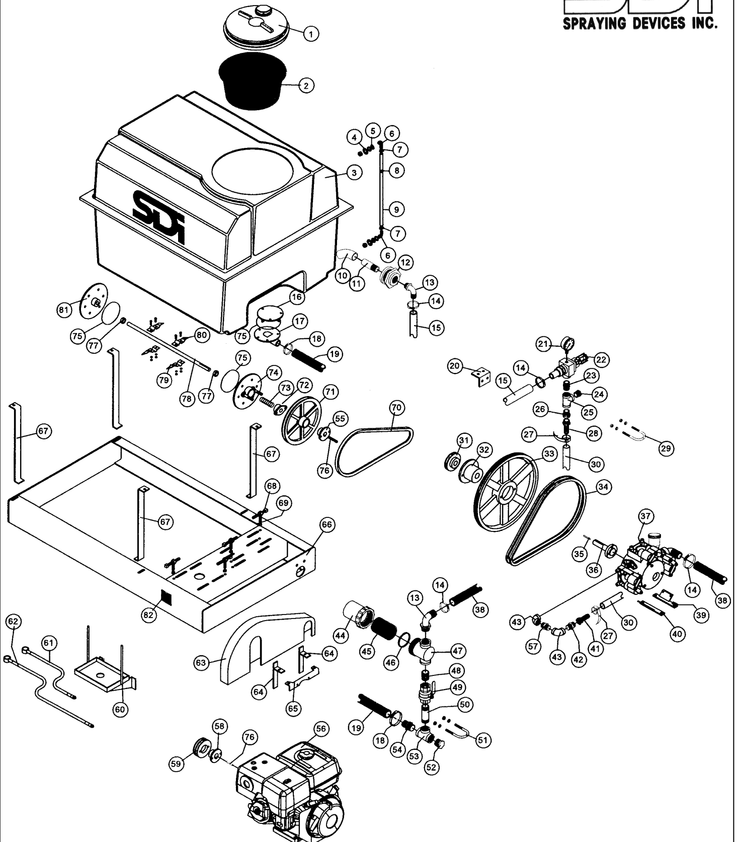
SDI Sprayer, Model 100-11HE6M
