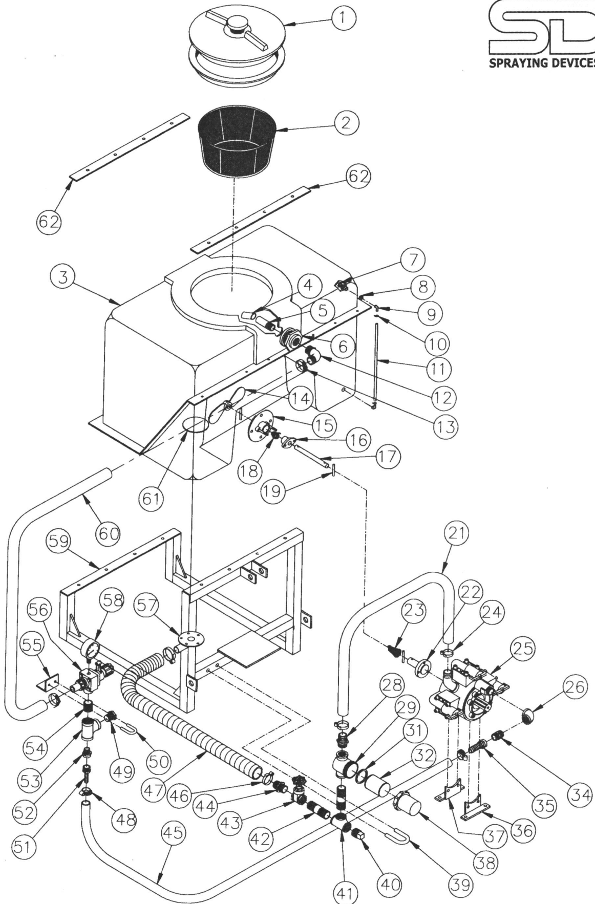
SDI Sprayer, Models 100 and 150-11P3PT
