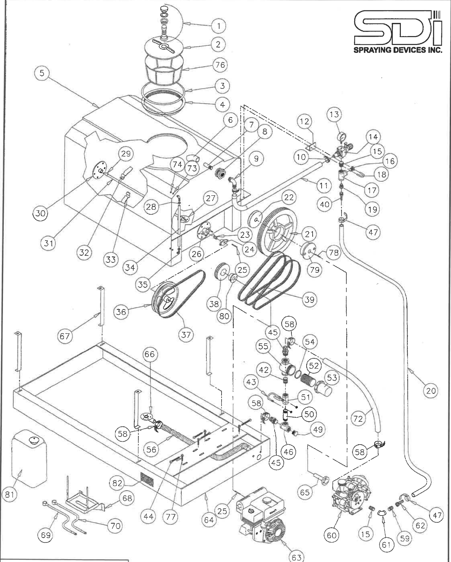
SDI Sprayer, Model 300-26KE20M
