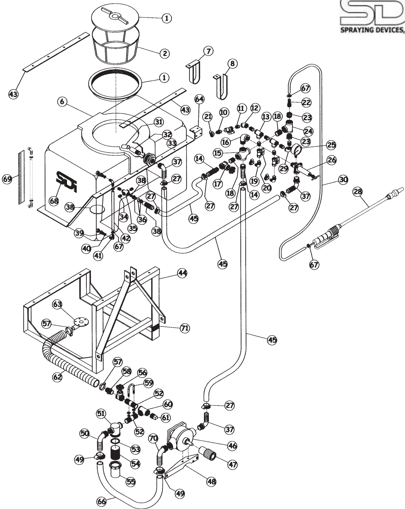
SDI Sprayer, Model No. 3PT50C
