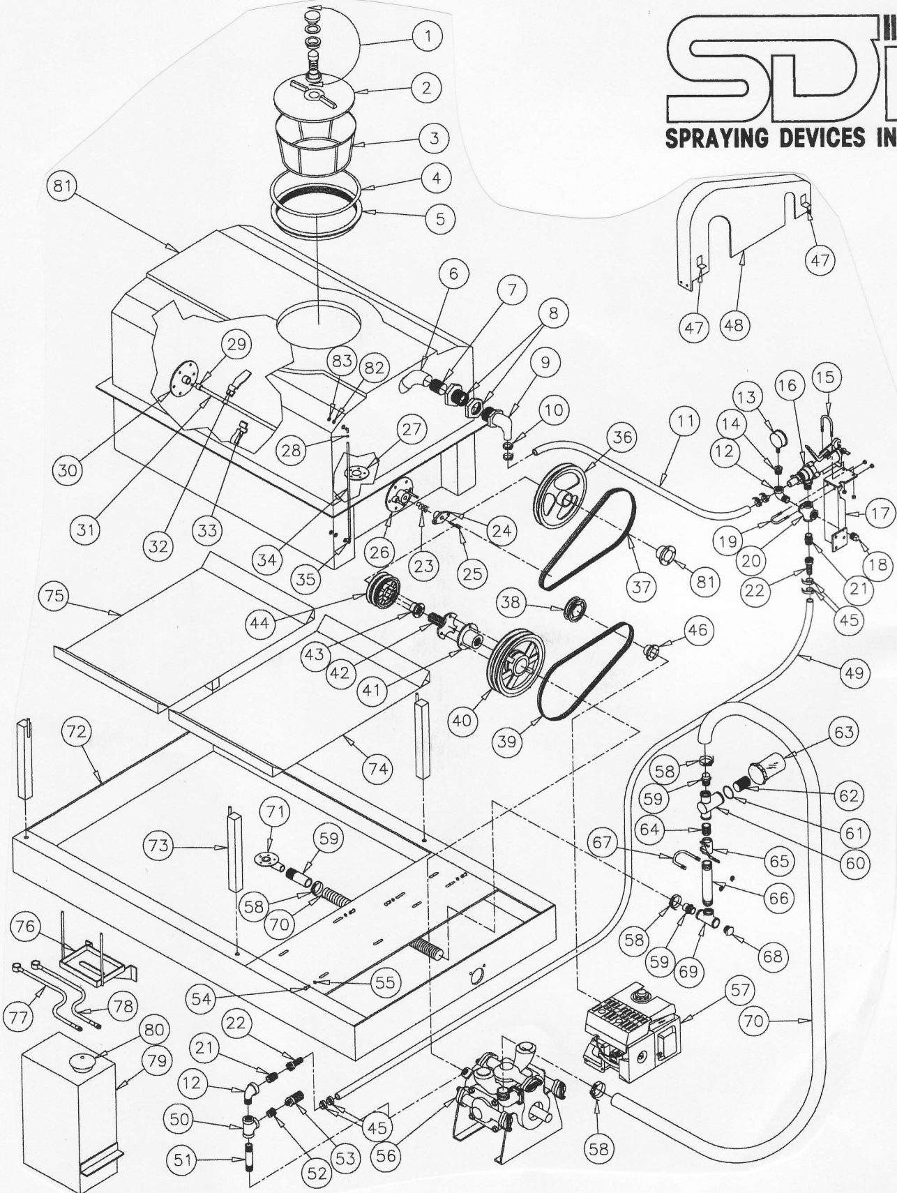
SDI Sprayer, Models 300, 500, 600 & 1000-38KE25M
