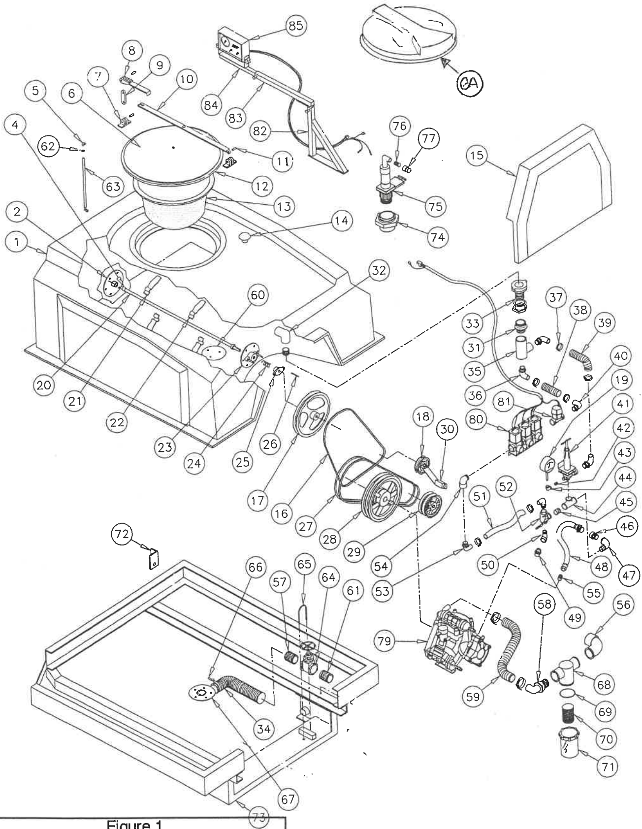
Figure 1 SDI Sprayer, Cushman, Diaphragm Pump P/N891387/891632 & 889897/891631
