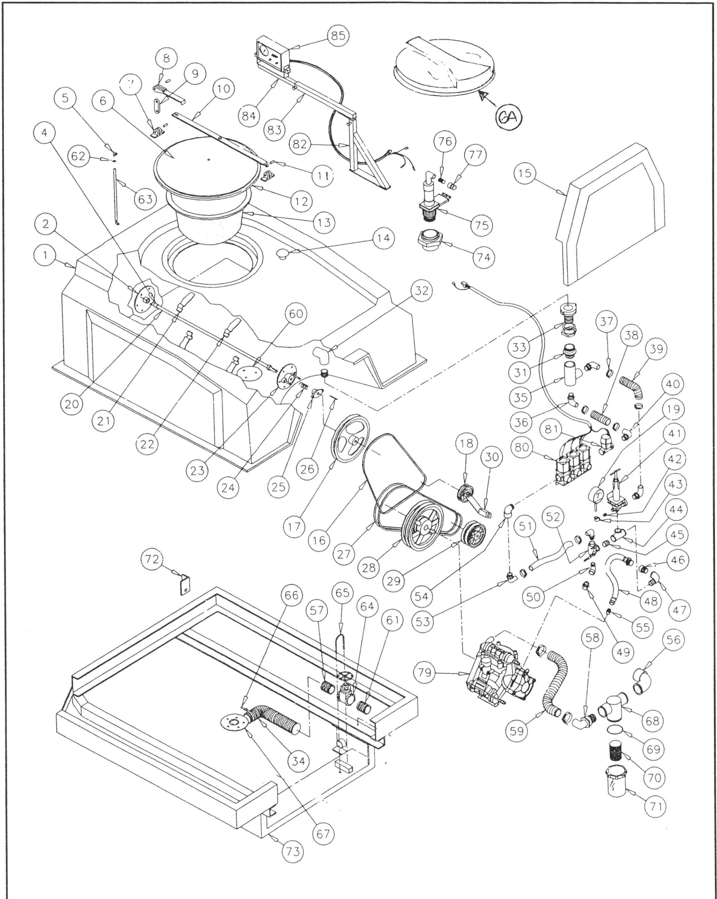
Figure 3 SDI Sprayer, Cushman, Diaphragm Pump P/N 891387/891388 & 889897/891388
