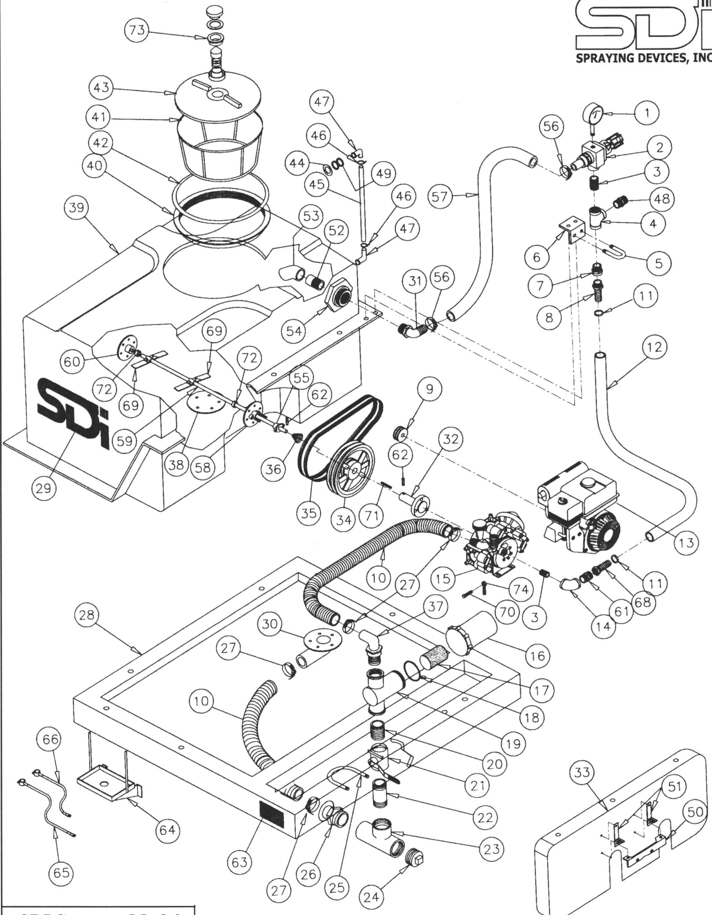
SDI Sprayer, Model PCO100-20HE5M
