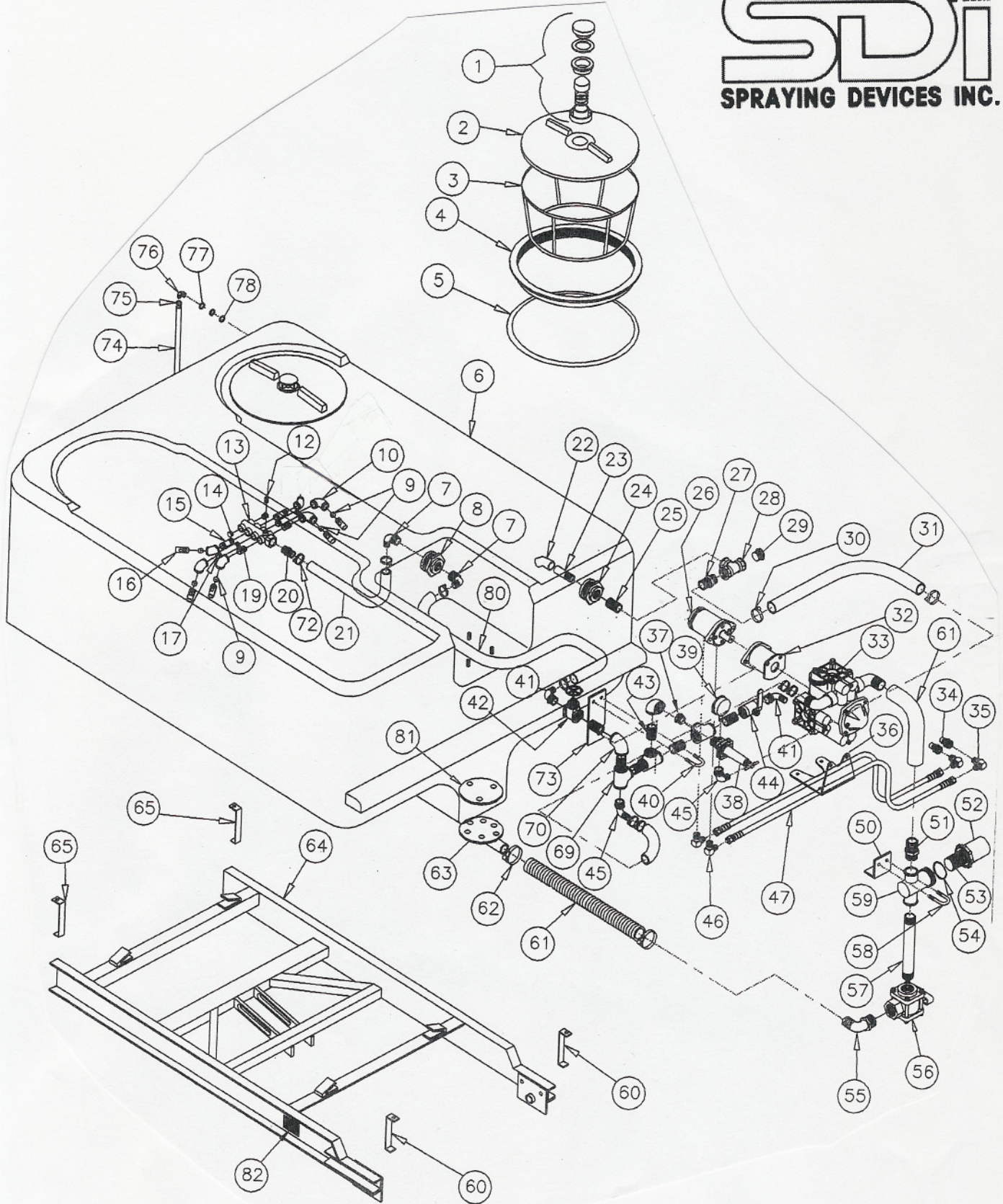
SDI Sprayer, Models PG160/PG225 & PG300
