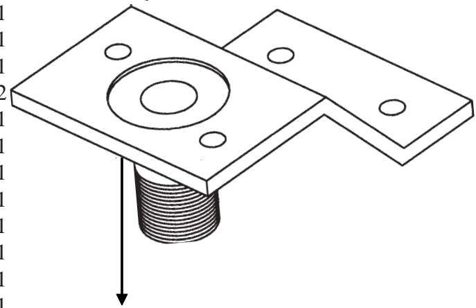
Part No. 11-147 - SDI Mounting Bracket for 9910-1923 Relief Valve.
