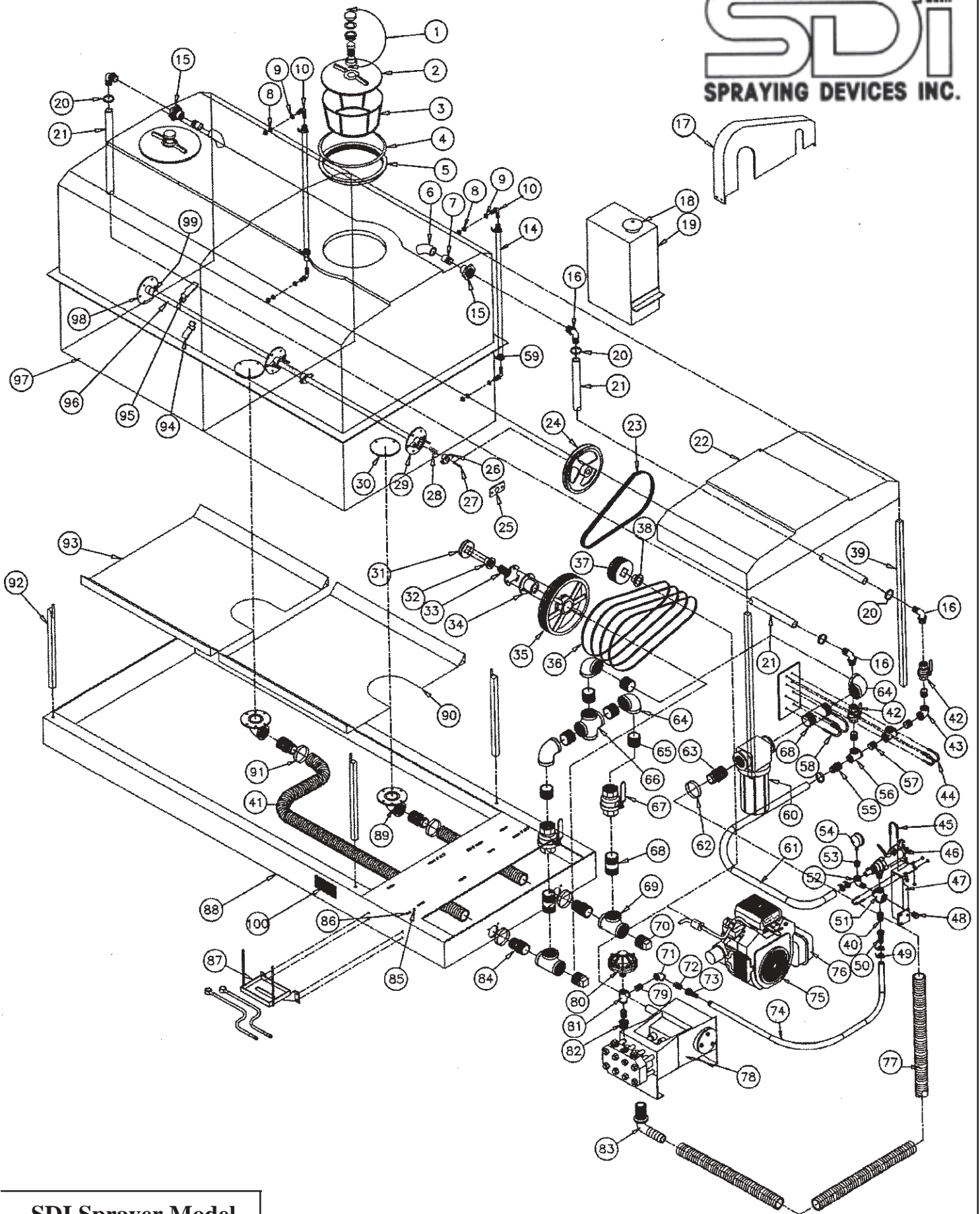
SDI Sprayer Model 600-JB35KE25M/Split
