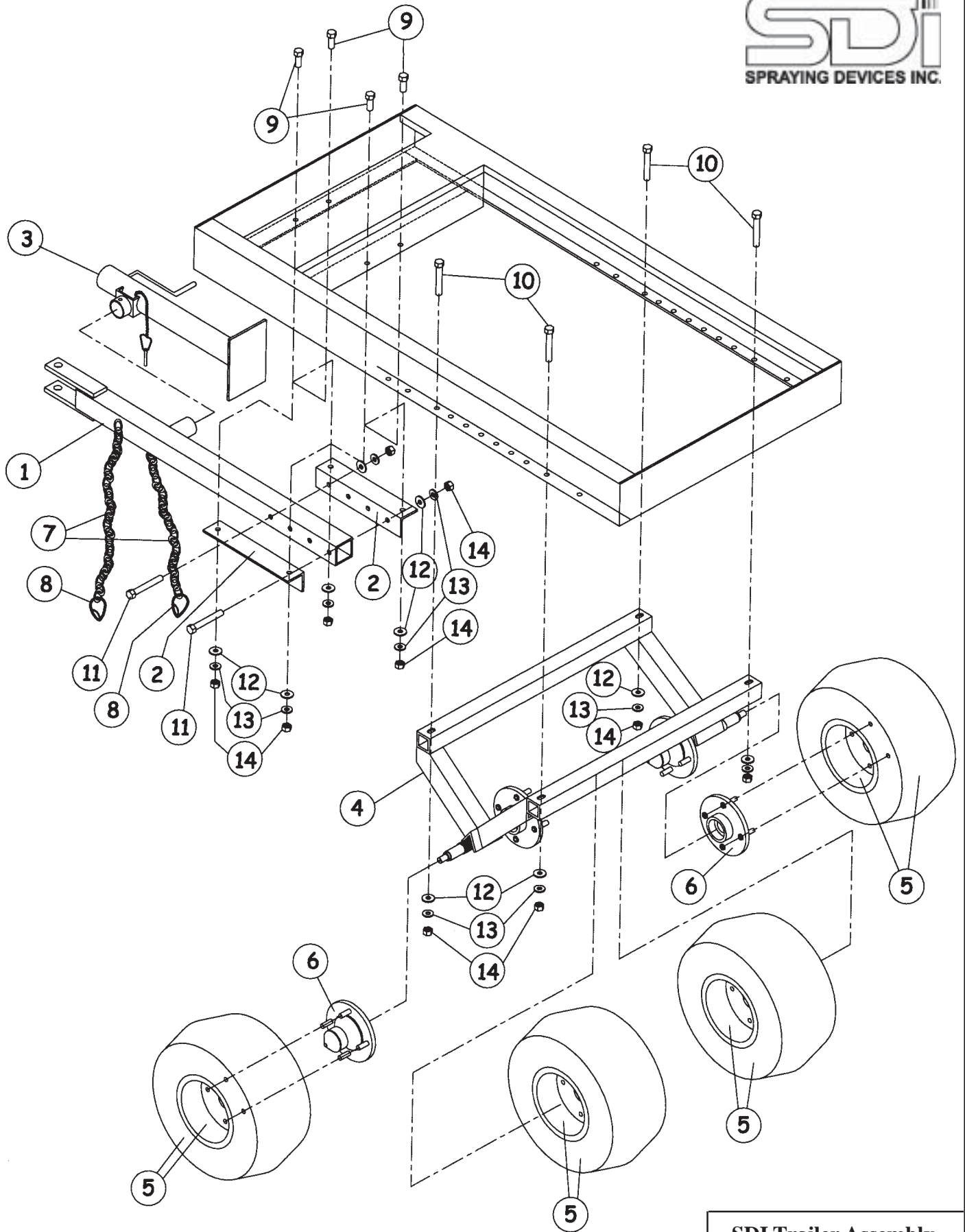
SDI Trailer Assembly Model TM80-22
