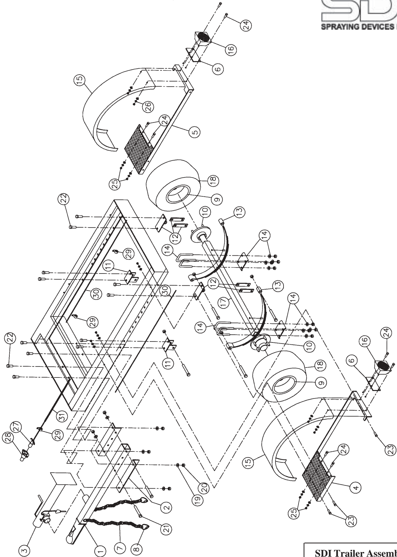
SDI Trailer Assembly Model TM80-24
