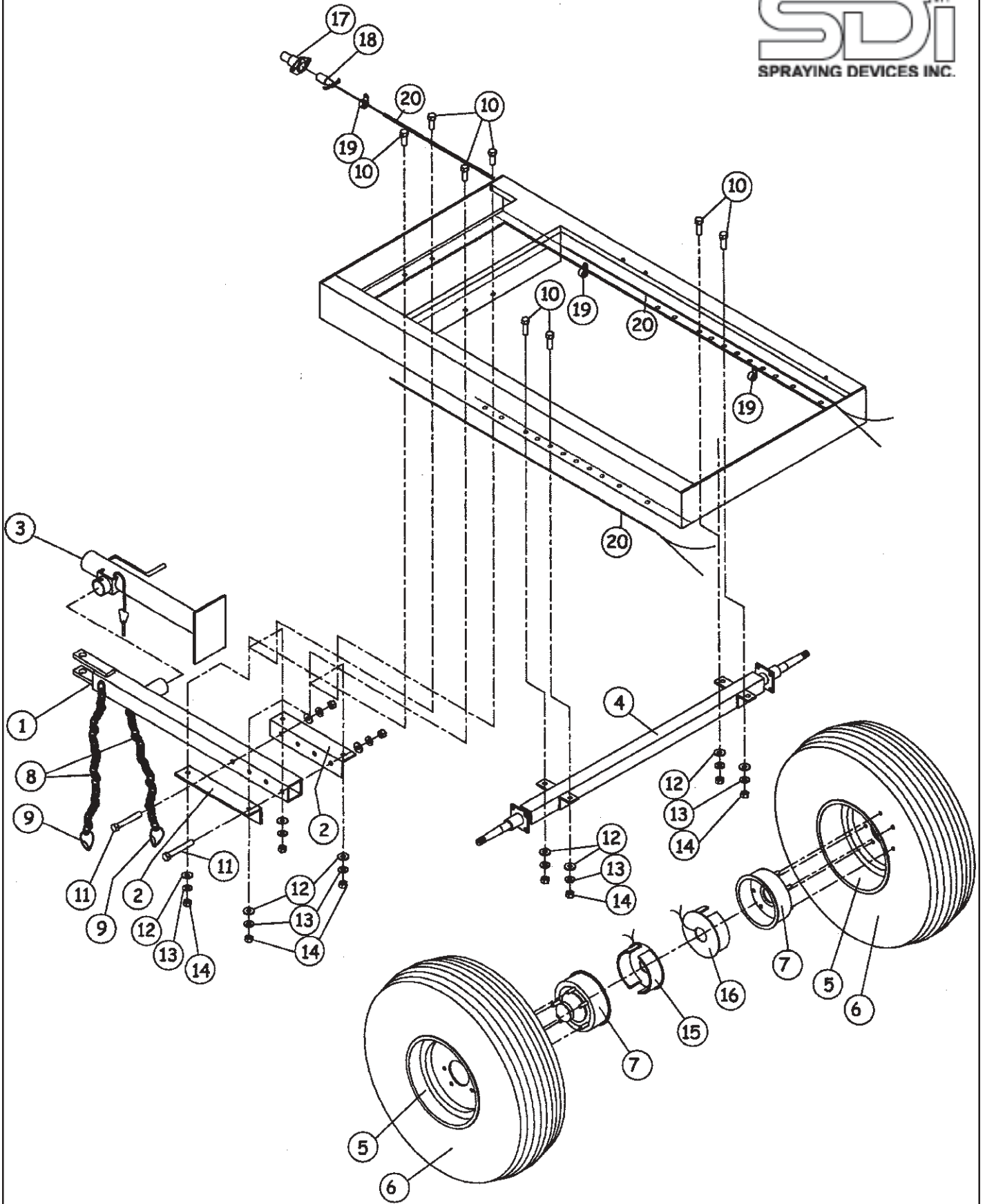
SDI Trailer Turf Assembly Model TM80-31E
