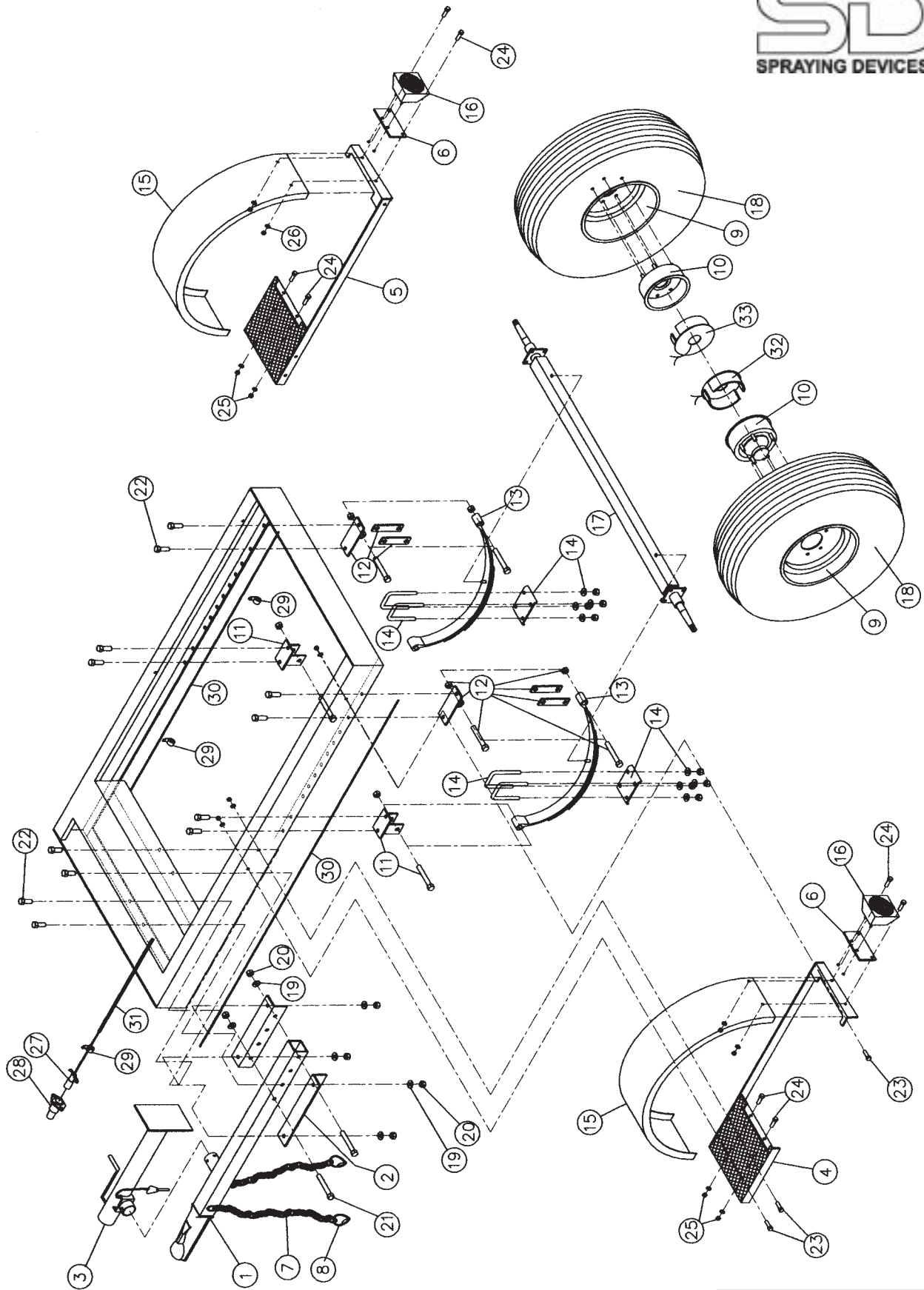
SDI DOT Trailer Assy W/Elec Brakes TM80-34E
