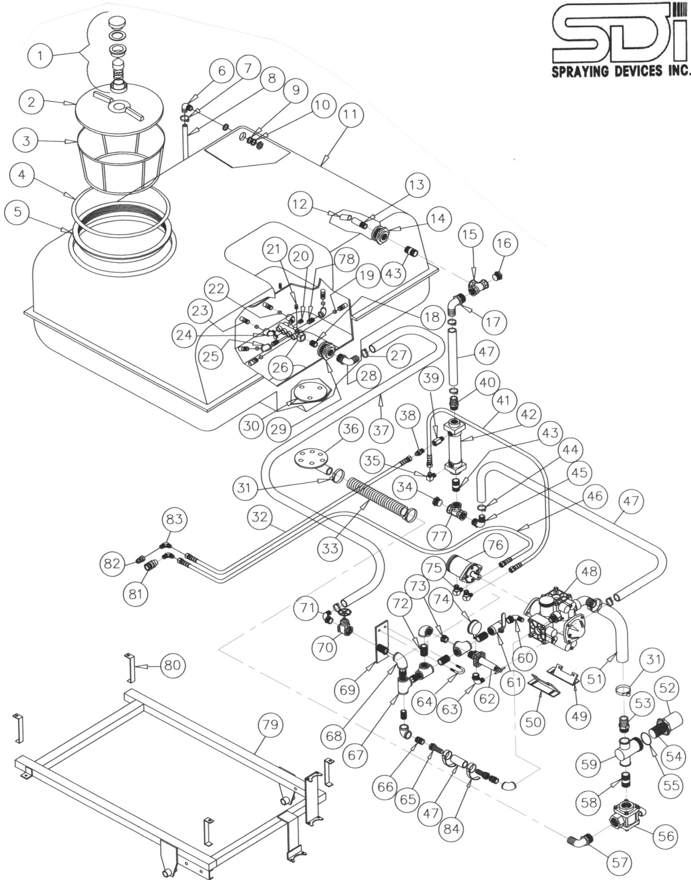
SDI Sprayer, Models VM160 & 225D/DSU
