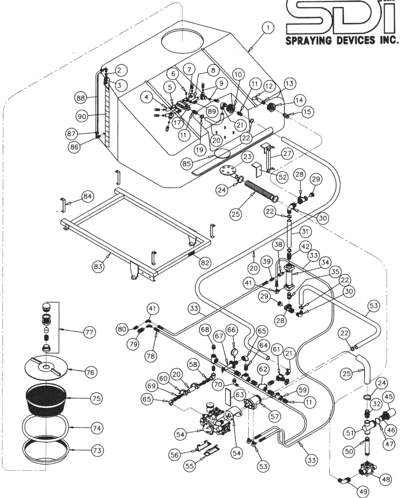
SDI Sprayer, Model VM300D/DSU
