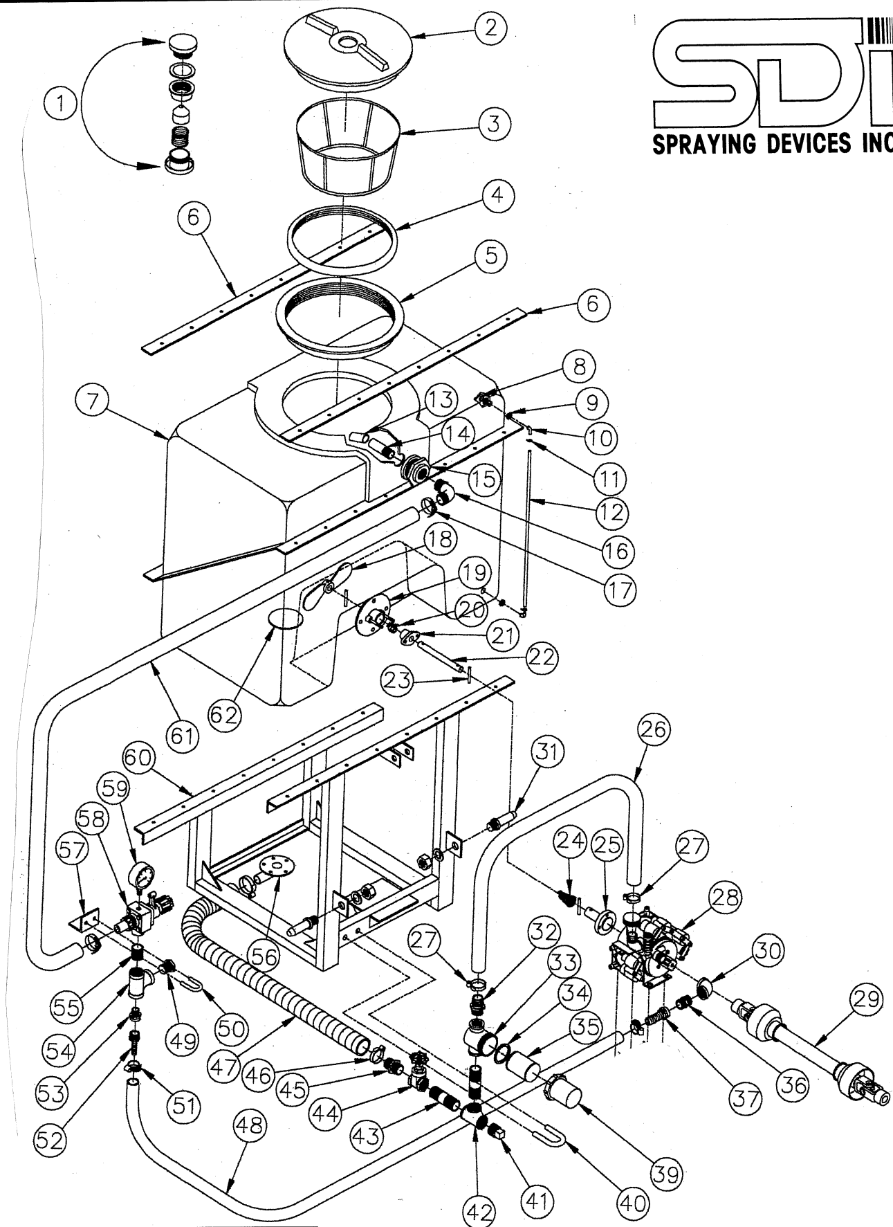
SDI Sprayer, Model No. 100 & 150-20P3PT
