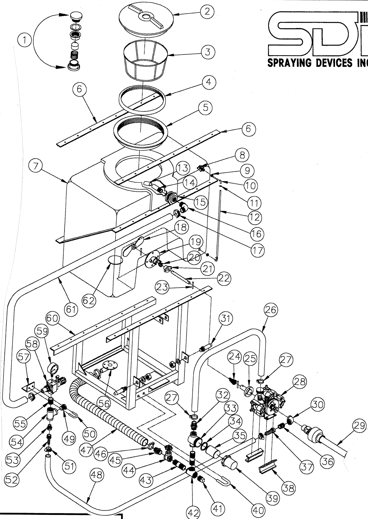
SDI Sprayer, Model No. 100 & 150-21P3PT
