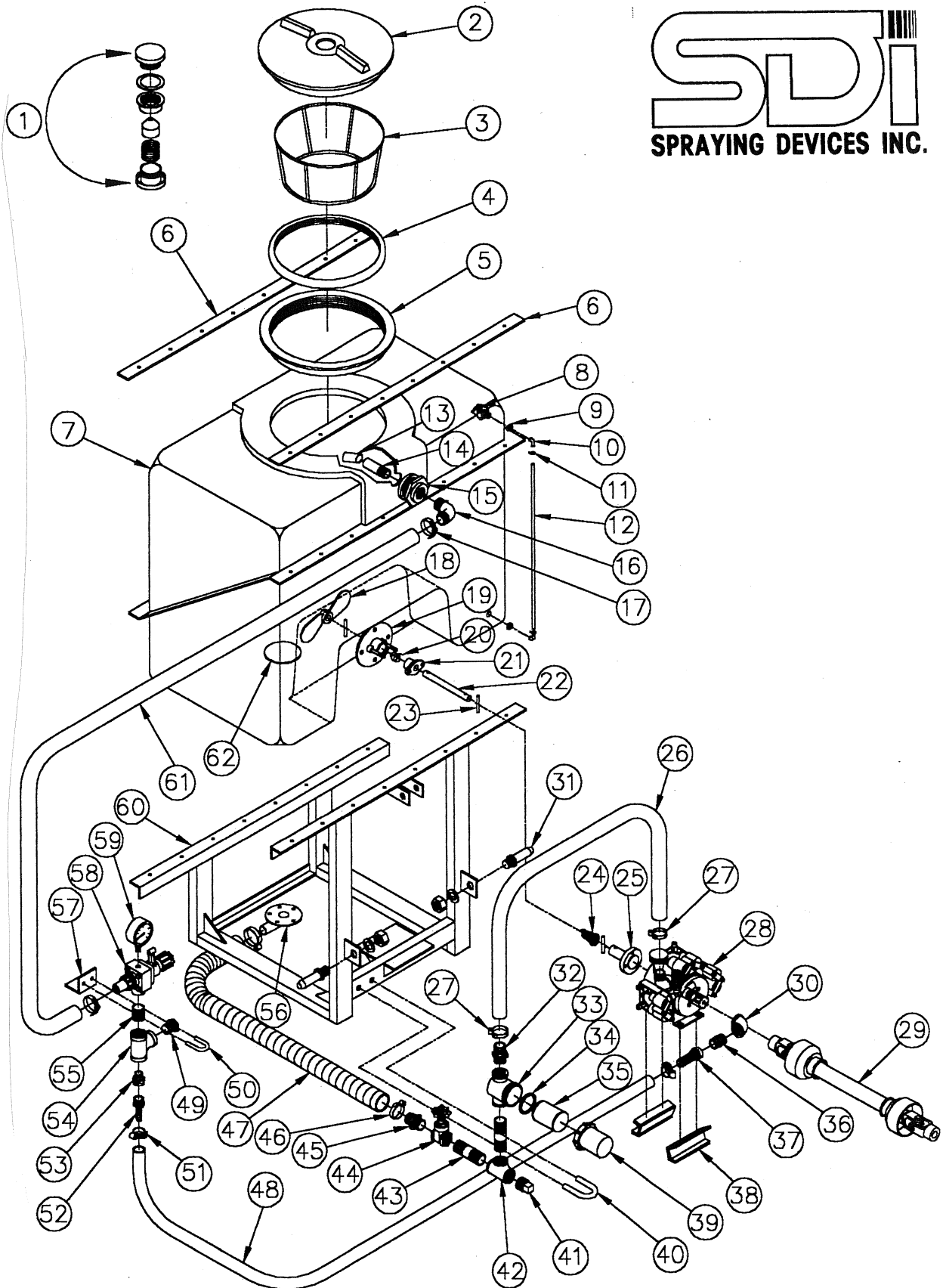
SDI Sprayer Model No. 150-24P3PT
