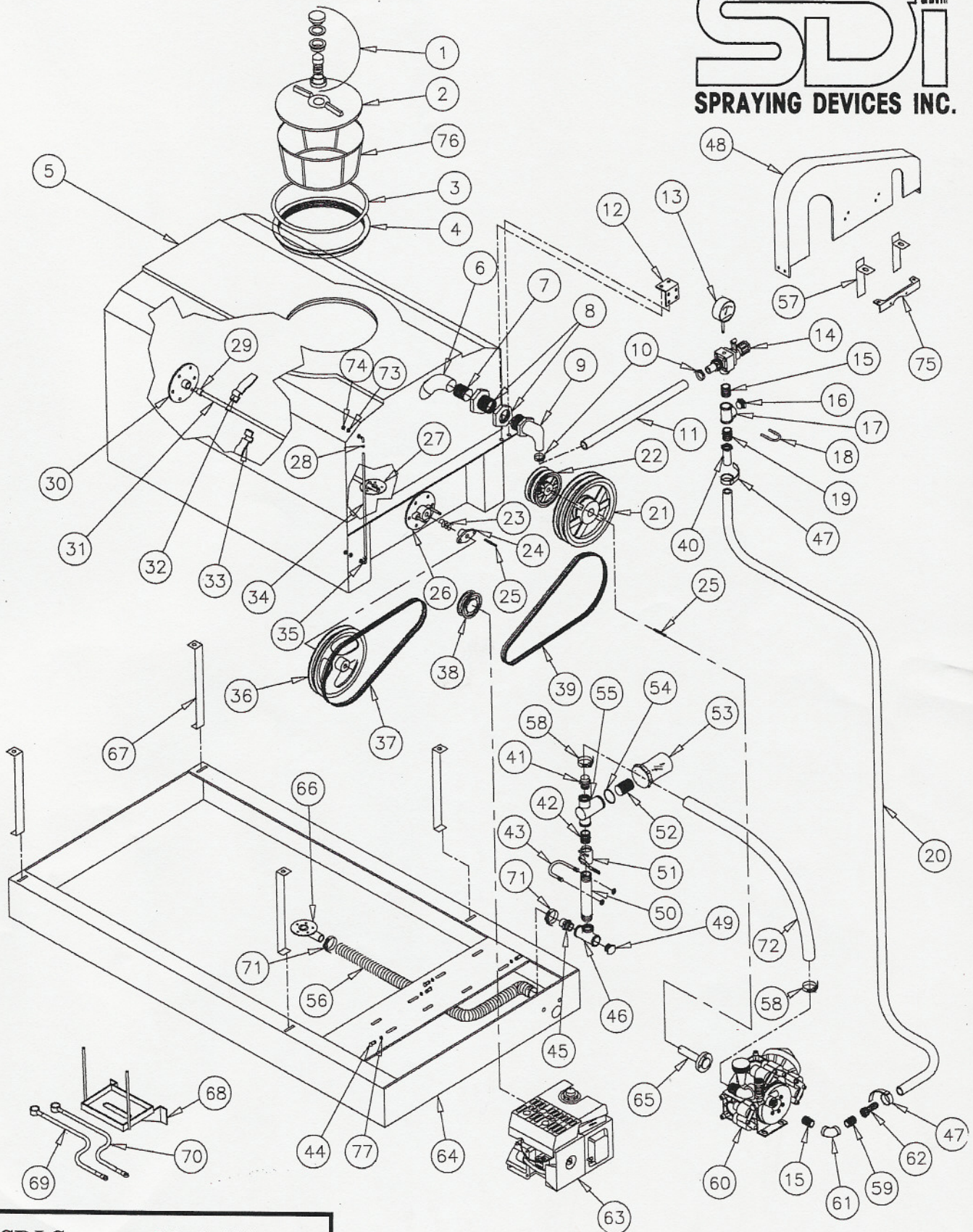
SDI Sprayer, Model No. 200-20HE13M
