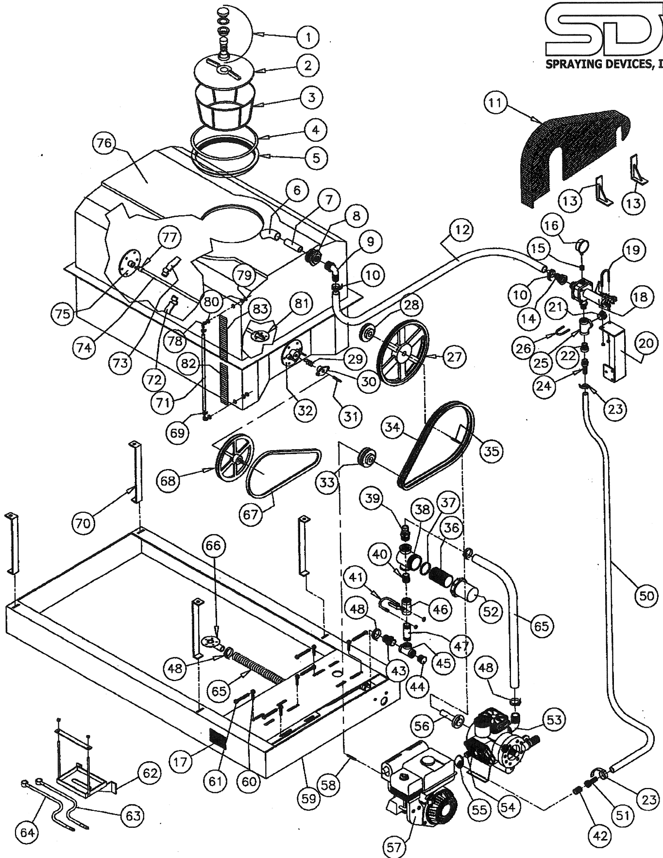
SDI Sprayer Model 200-21HE11M
