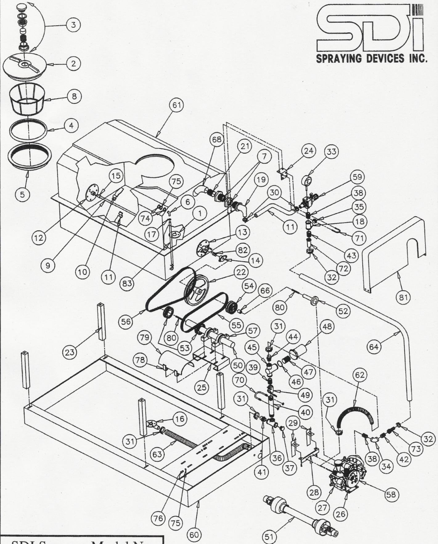
SDI Sprayer, Model No. 500-11PM
