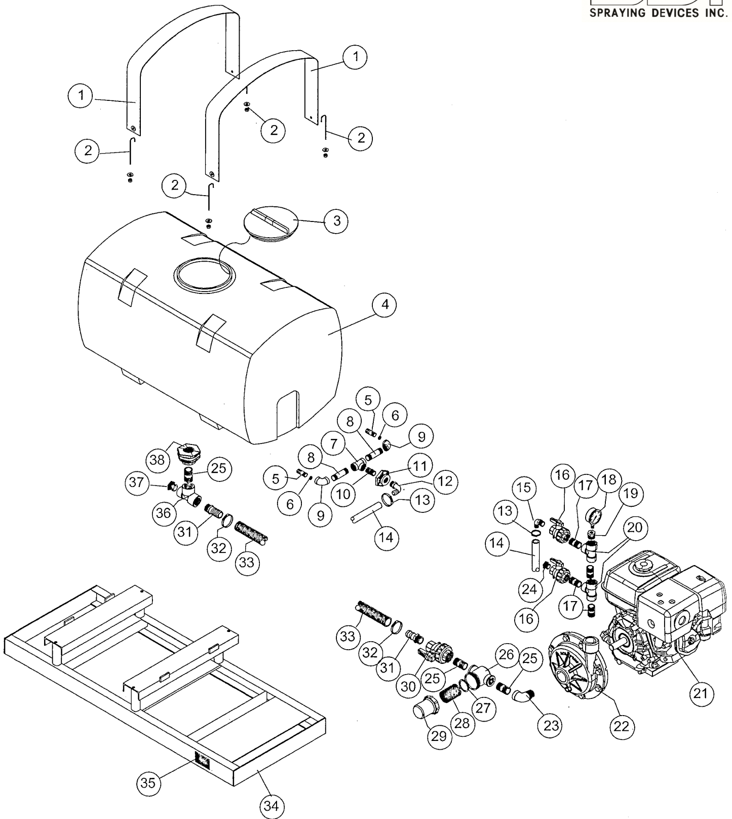
SDI Poly Sprayer 50PCO W/PE1685
