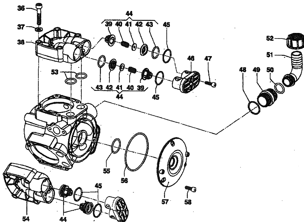
SDI Diaphragm Pump Part No. 78-00111
