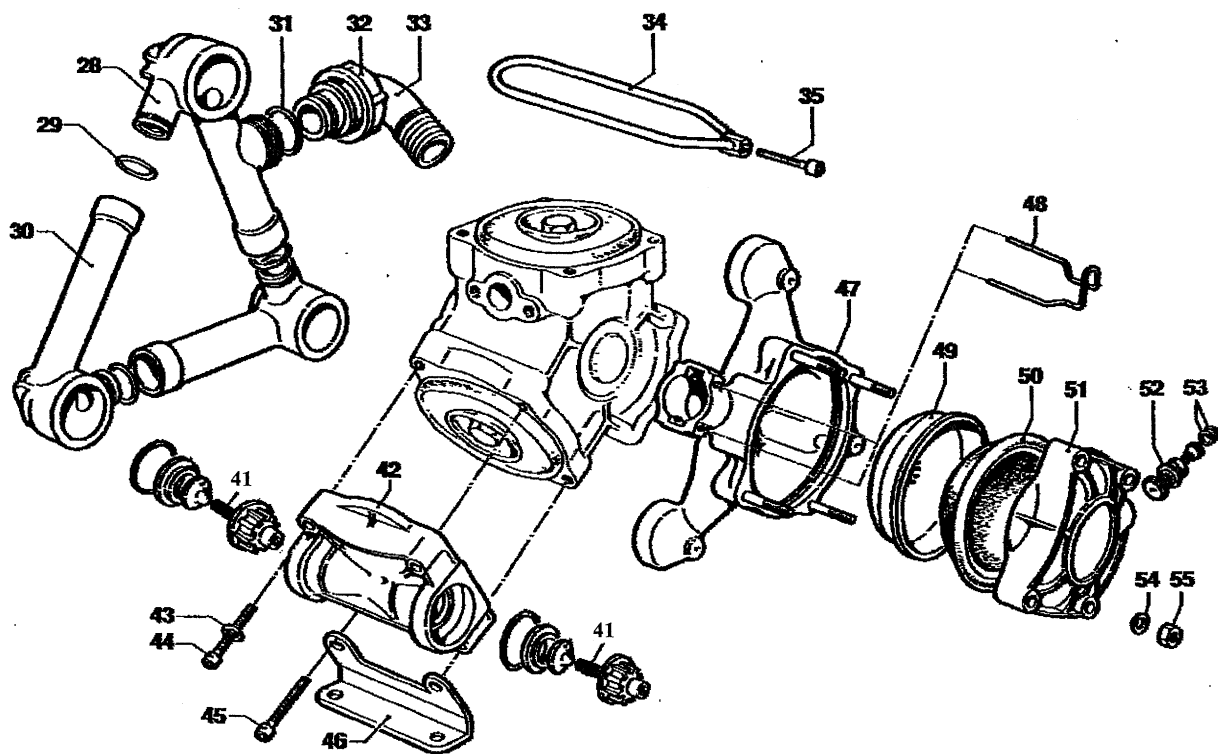
SDI Diaphragm Pump Part No. 78-0030
