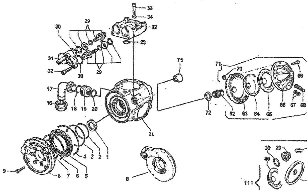
SDI Diaphragm Pump Part No. 78-020/78-0020
