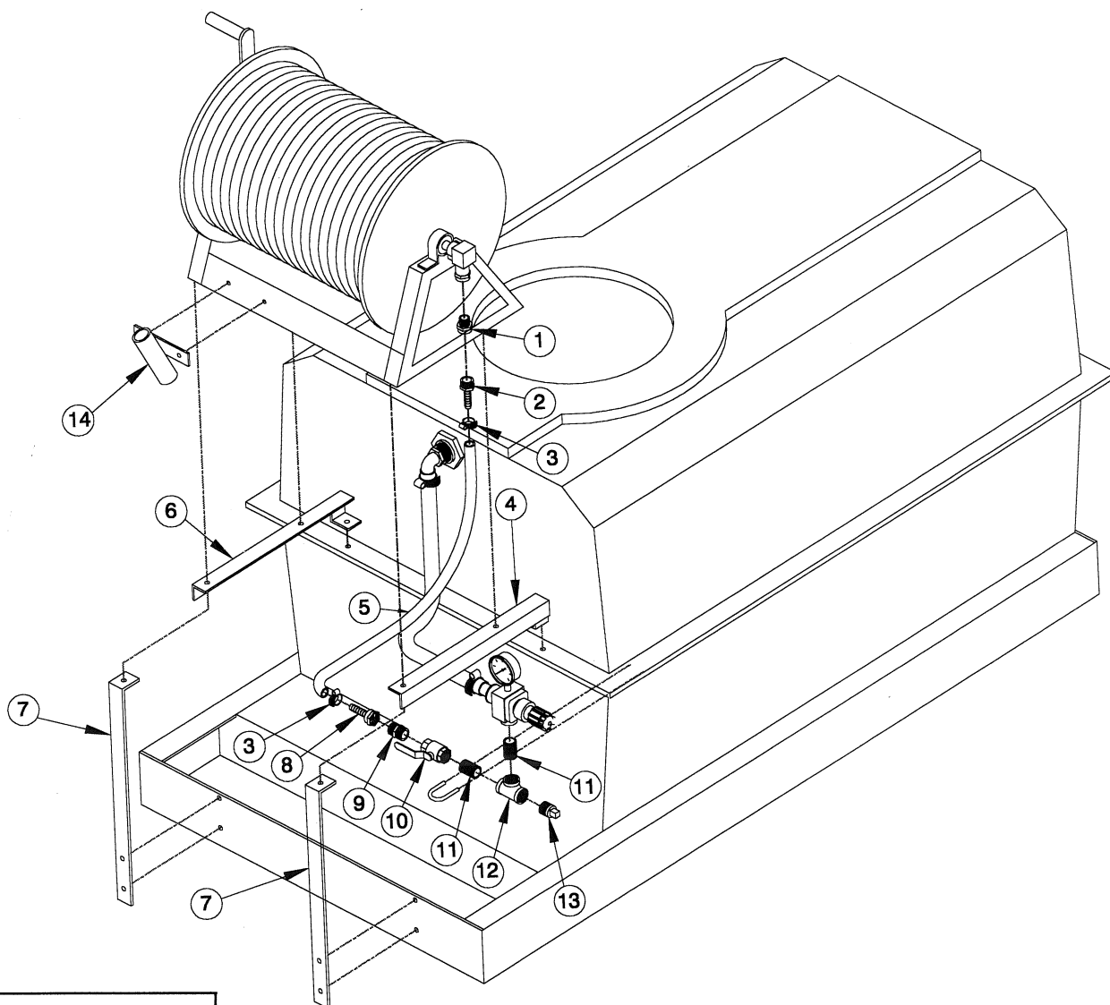
SDI Hose Reel Mounting Bracket Part #81-131
