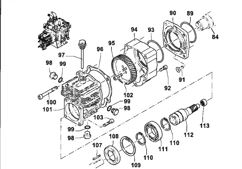
Figure 7. 9910-D70GR Gear Box Components
