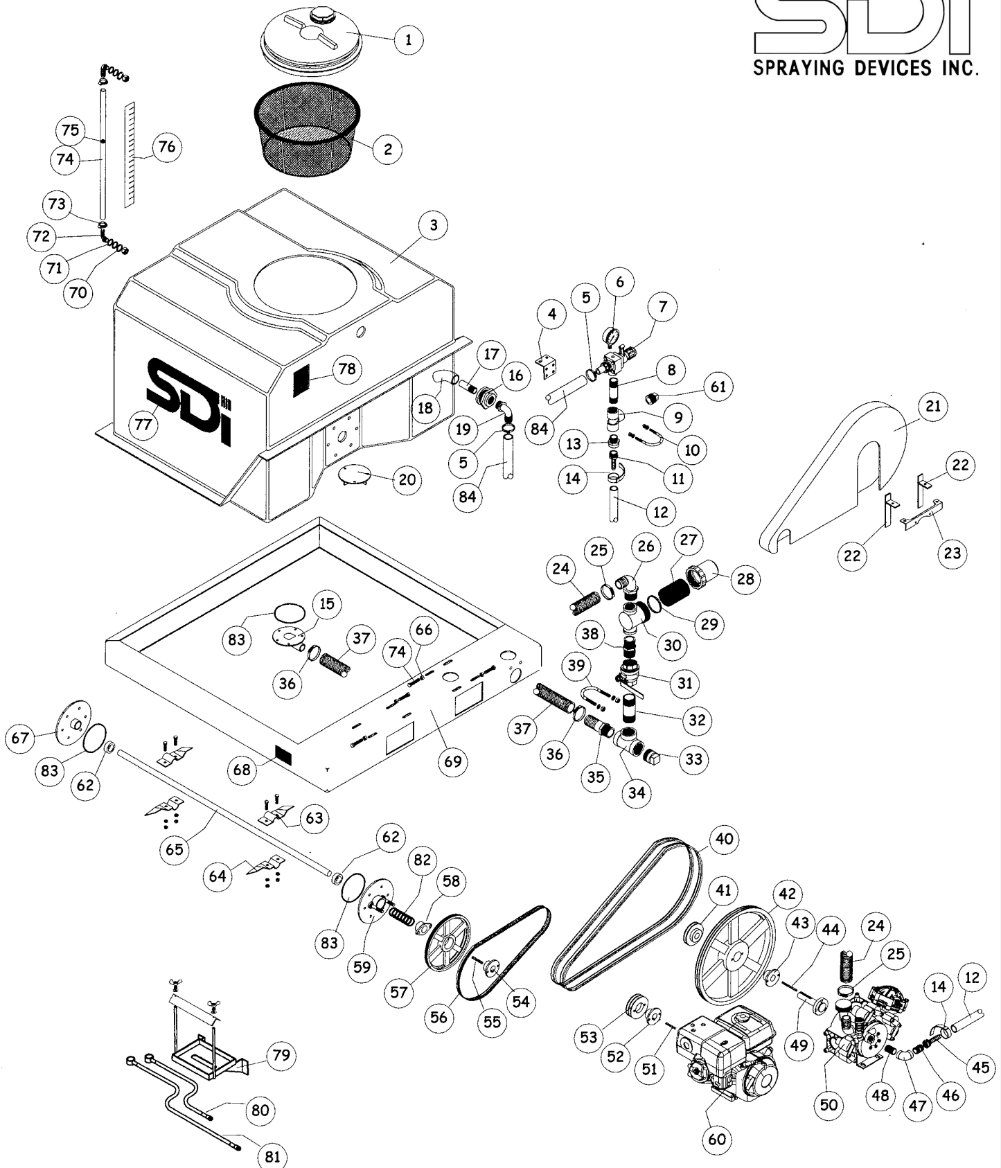
SDI Sprayer, Model No. C100 and C160-20H/HE6M
