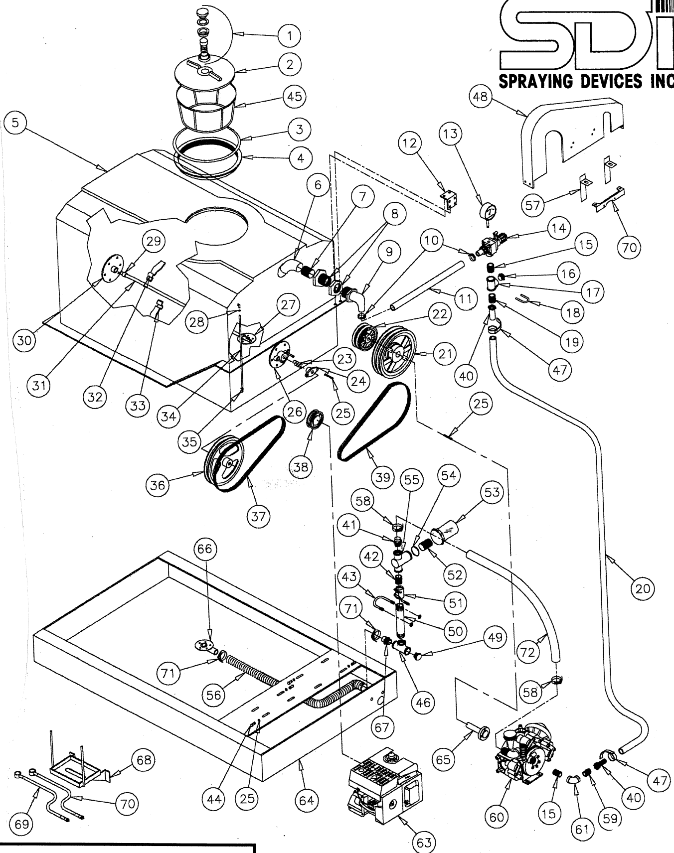
SDI Sprayer, Model No. C160-20KE12M
