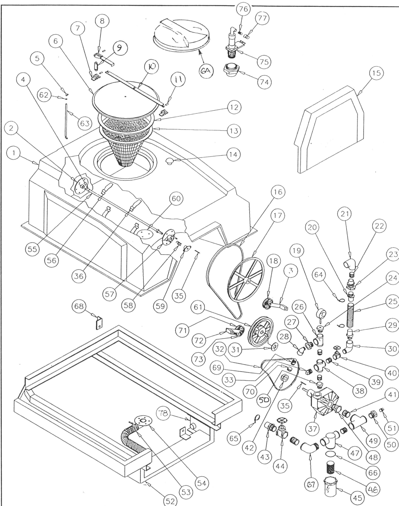
Figure 2 SDI Sprayer, Cushman, Centrifugal Pump P/N 891387 & 889897
