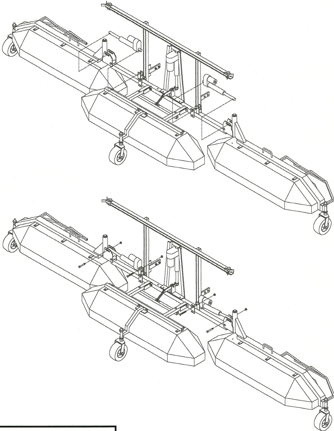
SDI Electric Lift Kit Part No. ELA KIT-2
