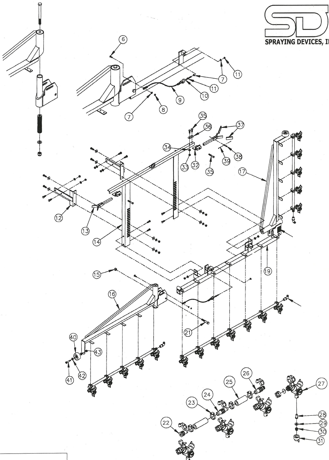
SDI Optimum Turf Spray Boom
