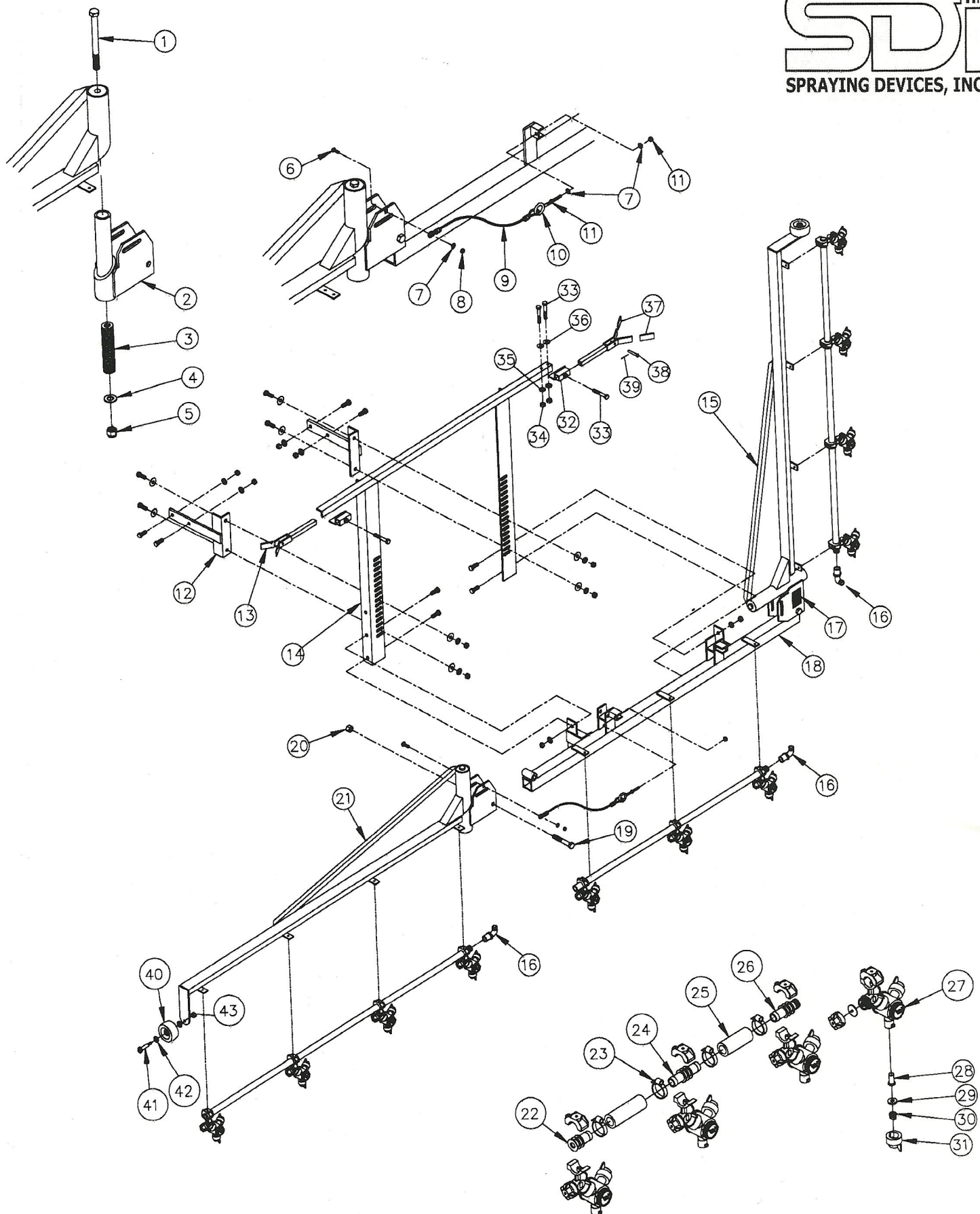
SDI Optimum Turf Spray Boom
