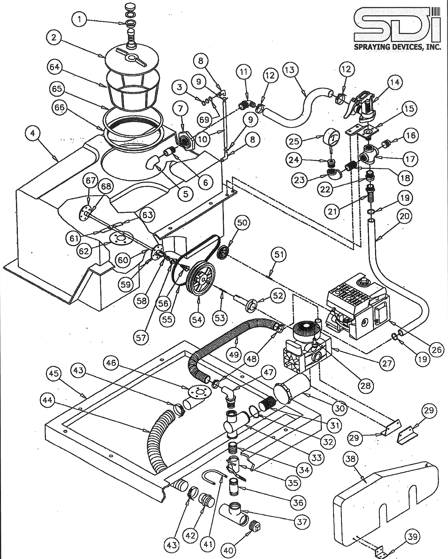
SDI Sprayer, Model PCO100-9K6M
