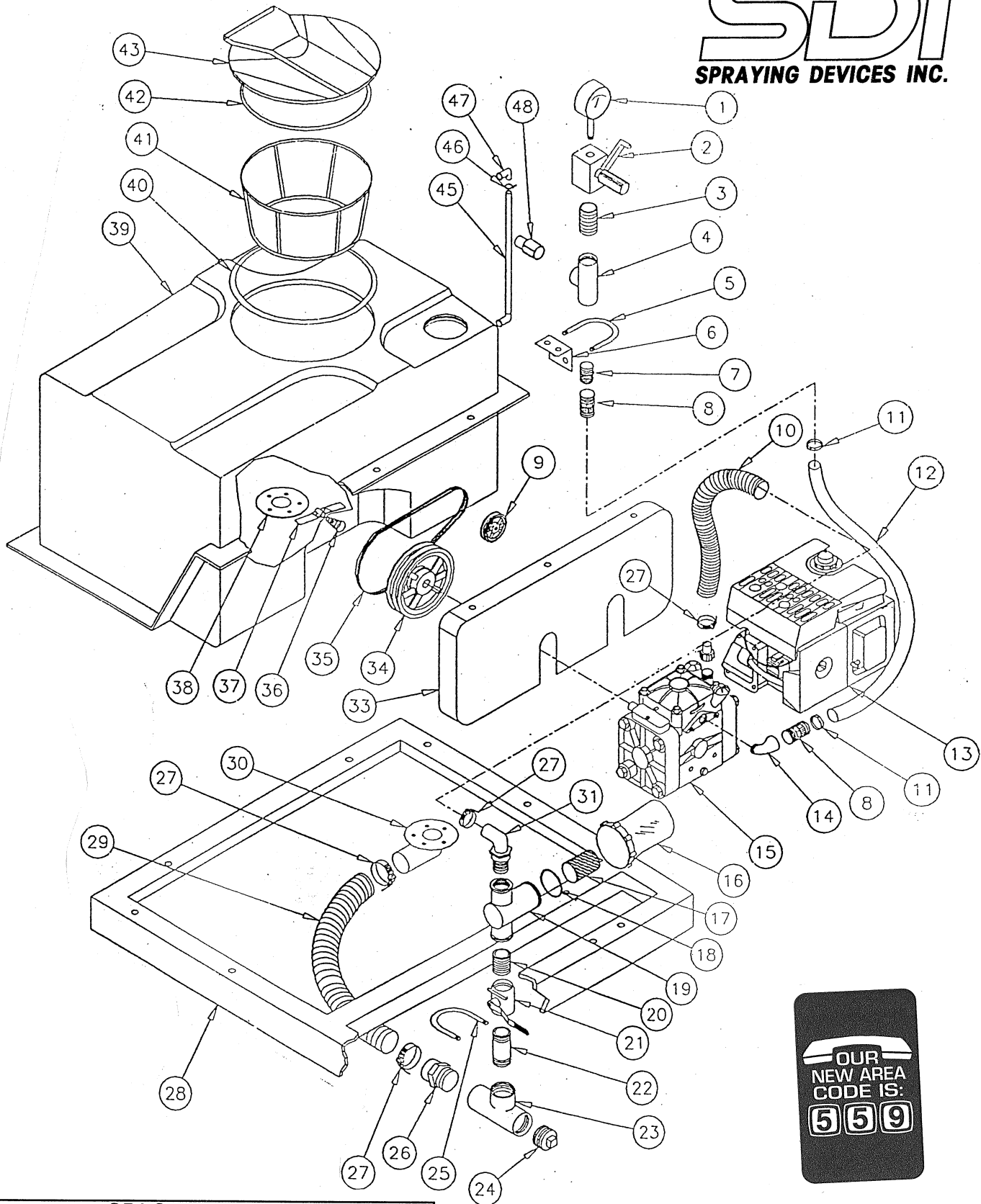
SDI Sprayer, Models PCO50-20K8M & PCO100-20K8M
