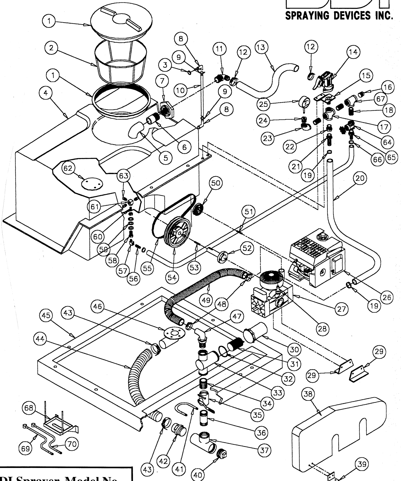
SDI Sprayer, Model No. PCO50-9H & 9HE5J
