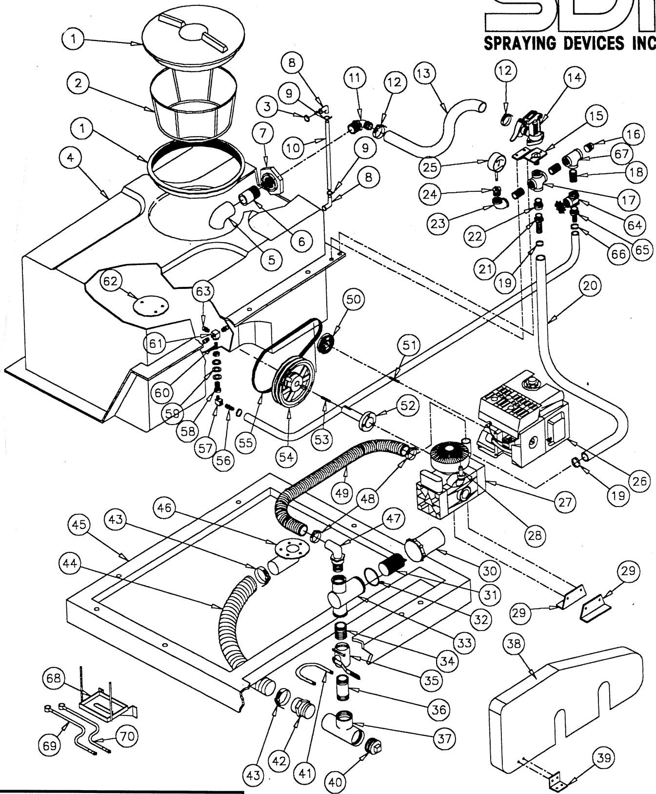
SDI Sprayer, Model PCO50-9K6J/9KE6J
