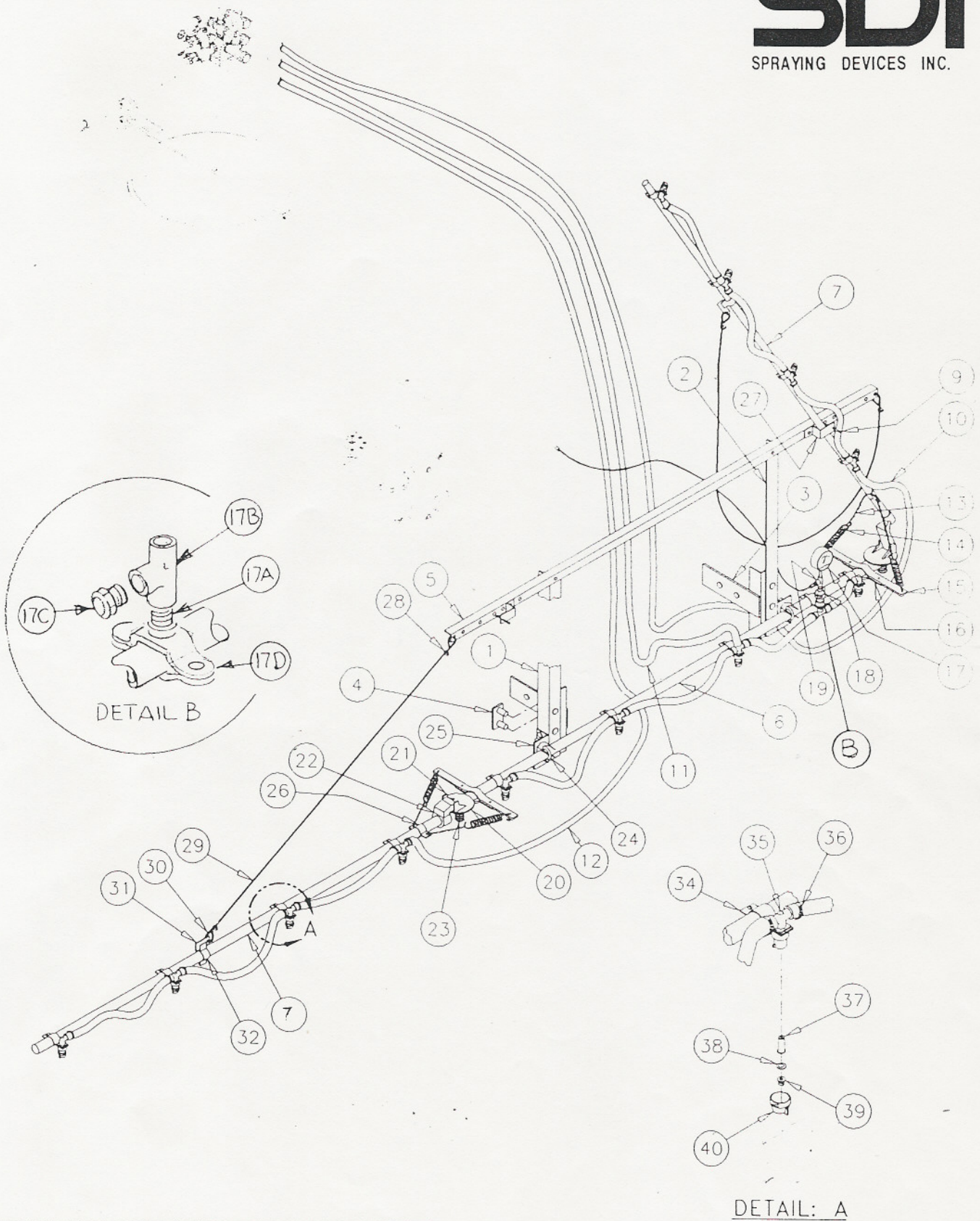
Figure 4 SDI Dry Boom Assembly, SB 20/20D
