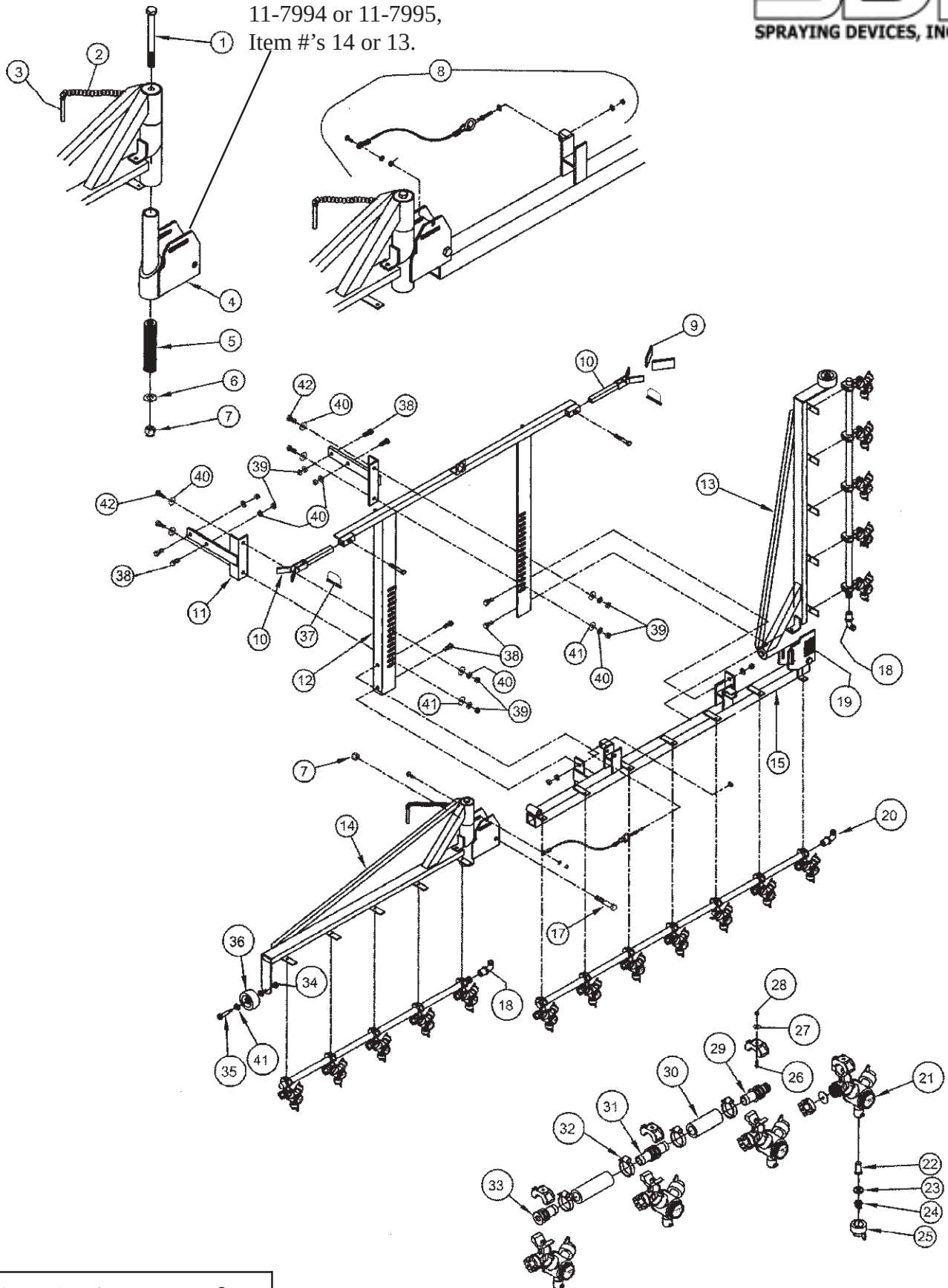
SDI Optimum Turf Spray Boom
