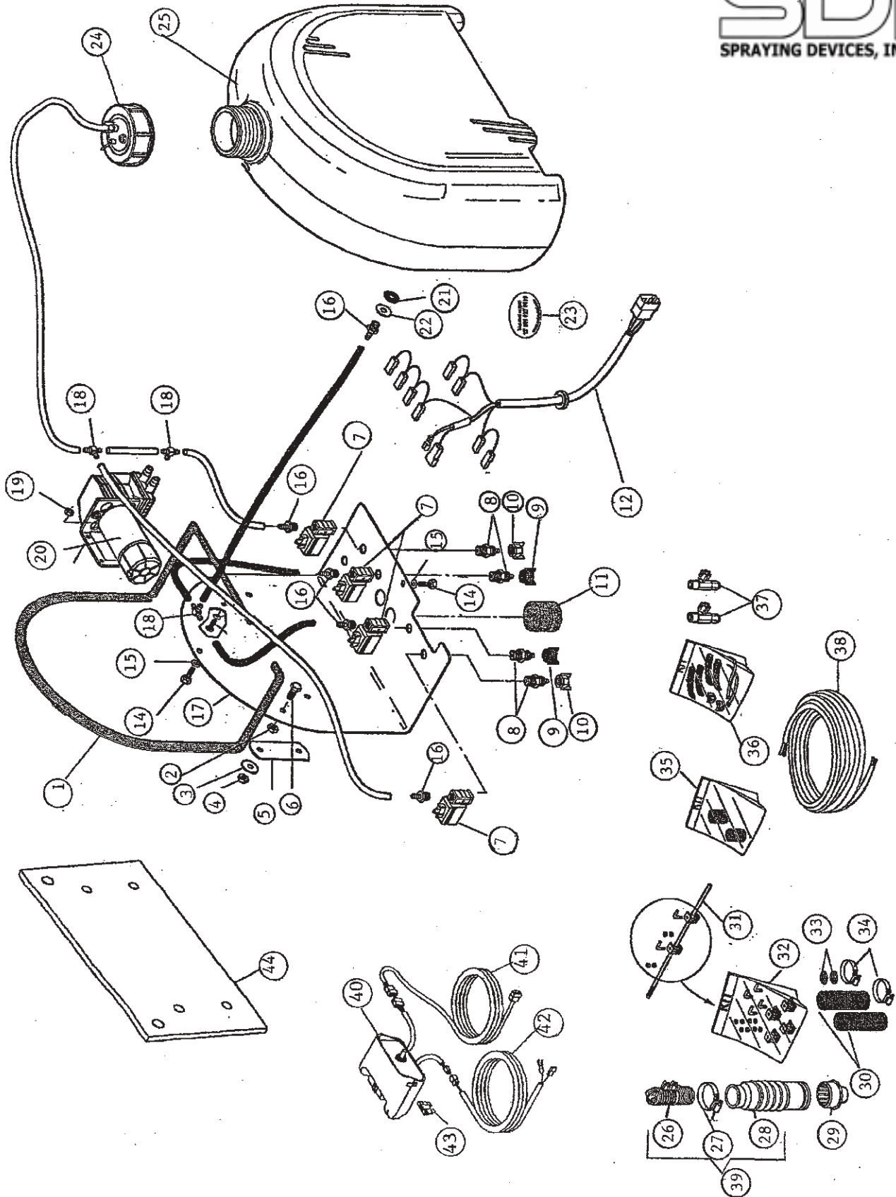
SDI Foam Marker System
