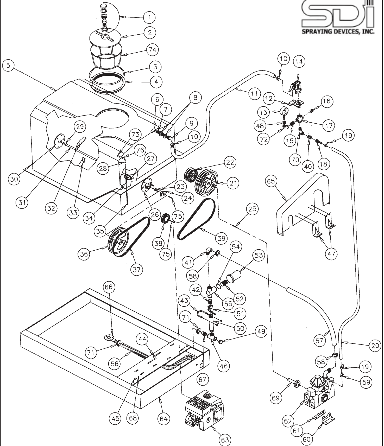
SDI Sprayer, Models C100/ C160-9K6M and 14K6M
