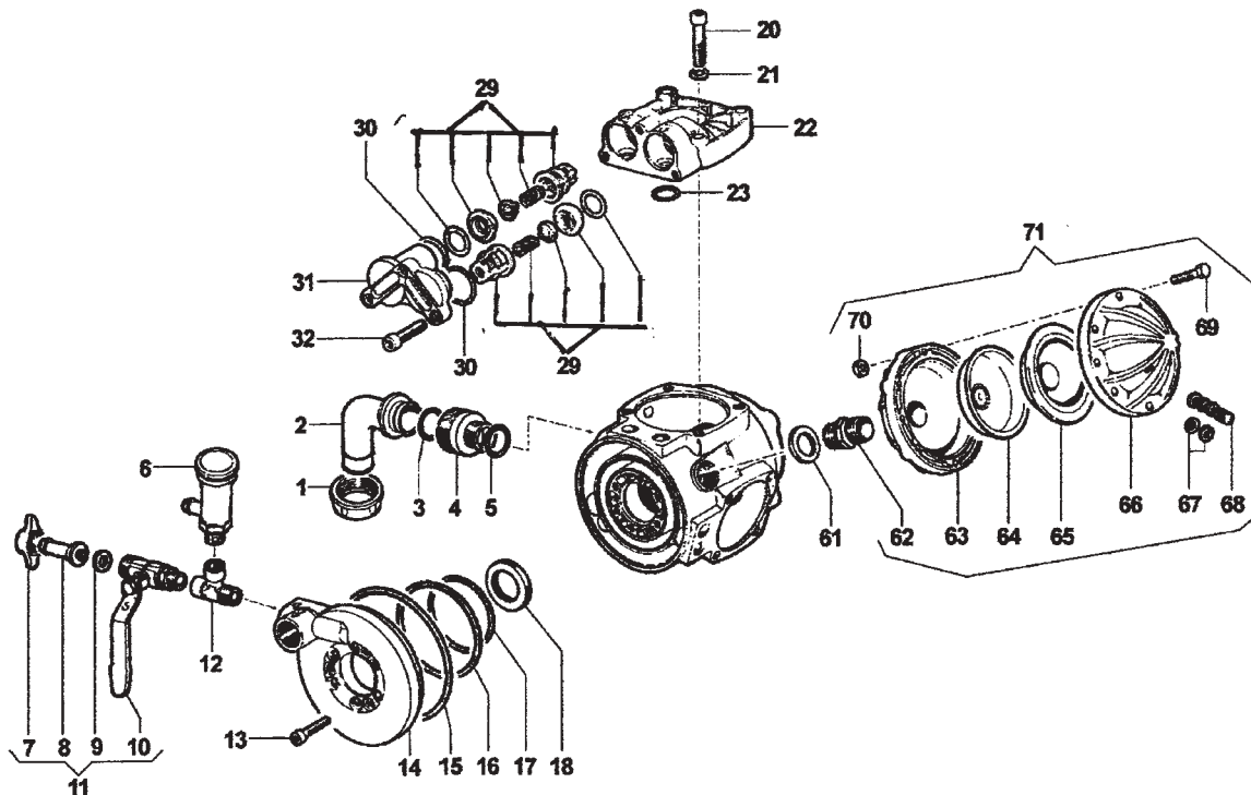
SDI Diaphragm Pump Part No. 78-0020
