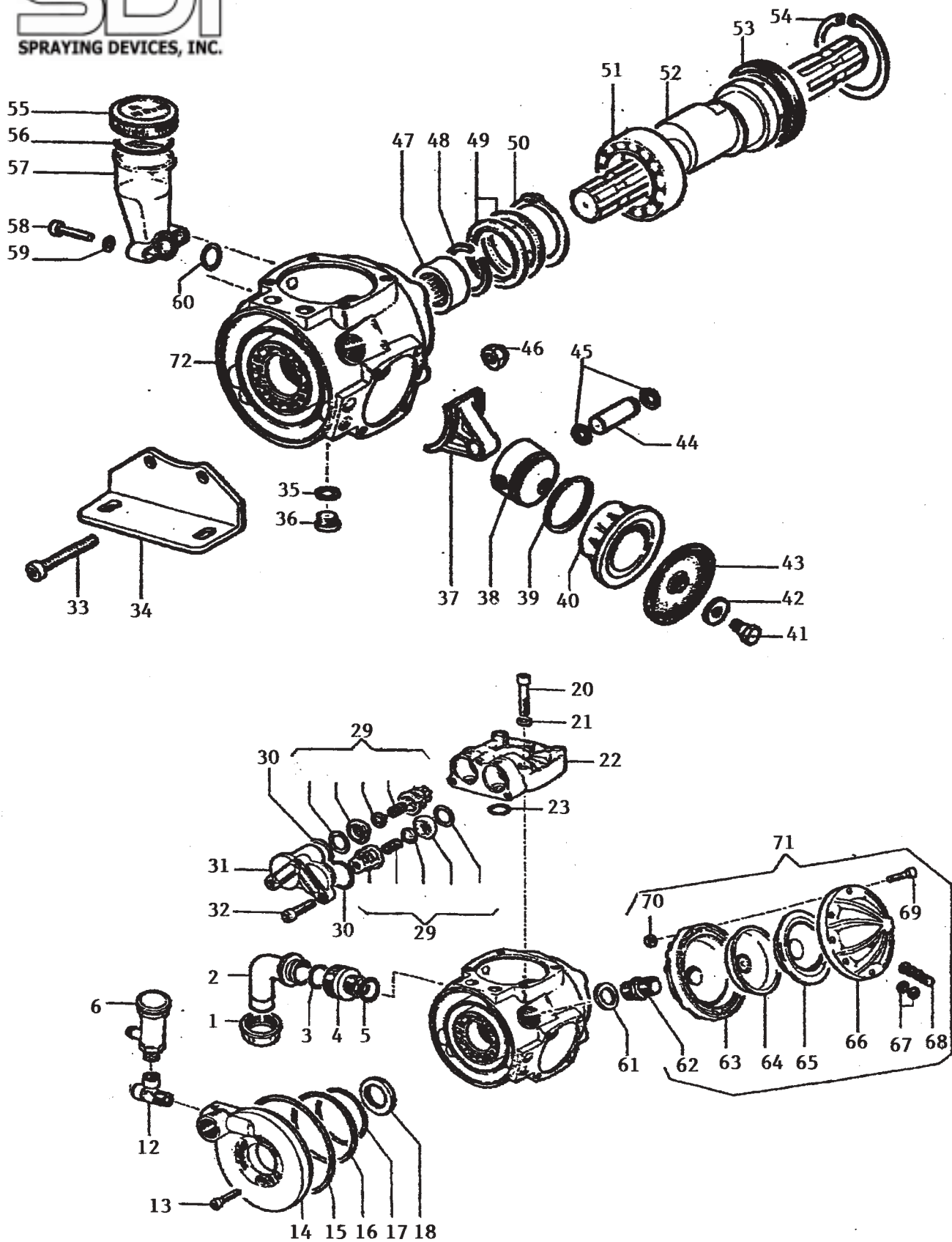
SDI Diaphragm Pump Part No. 78-0020AP
