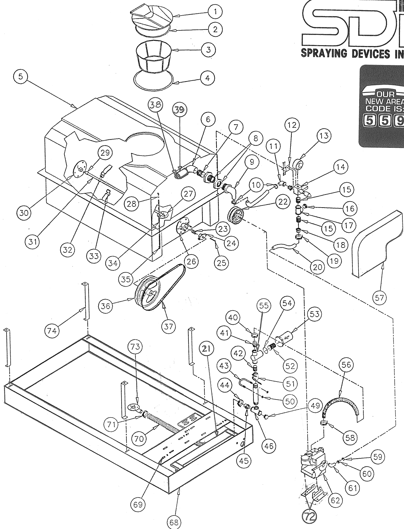
SDI SPRAYER MODEL TM 300H-C
