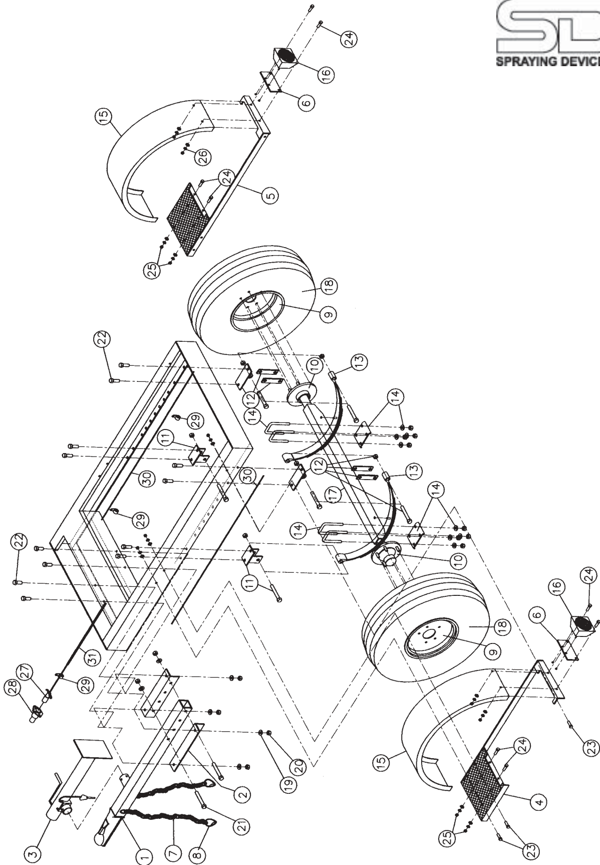
SDI DOT Trailer Assembly Model TM80-34
