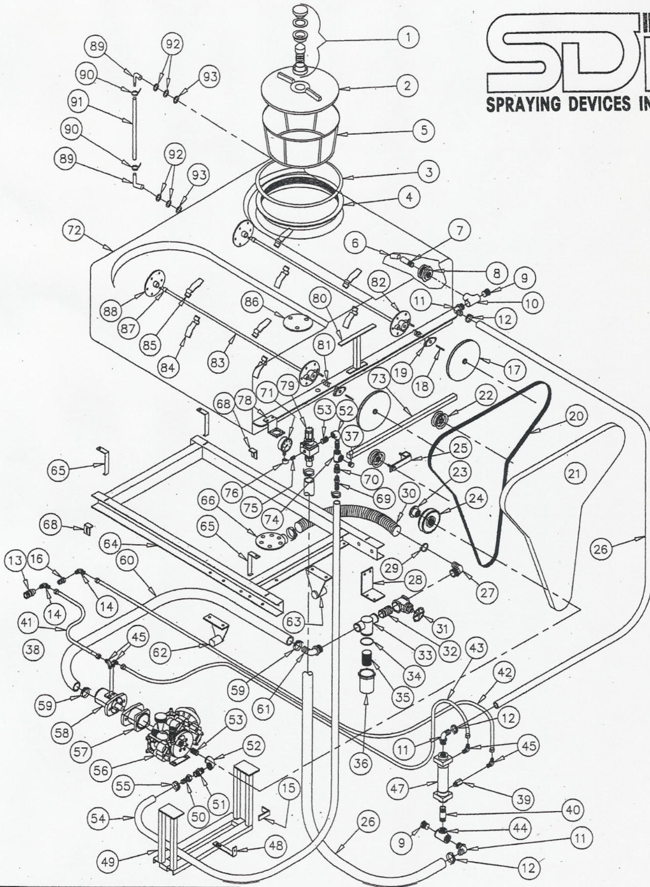
SDI Sprayer, Model No. VM200 & VM240H-C
