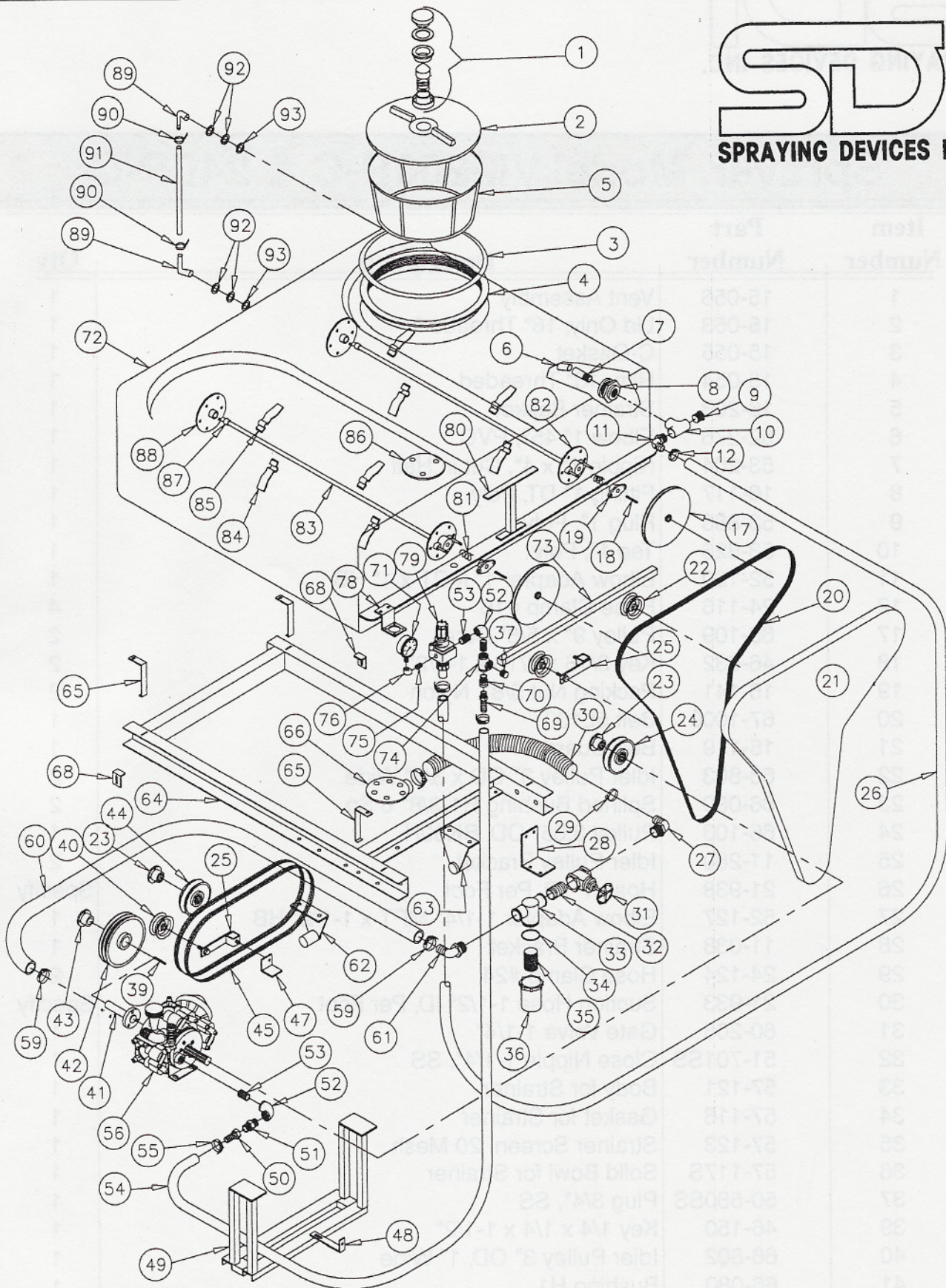
SDI Sprayer, Models VM200P-C & VM240P-C
