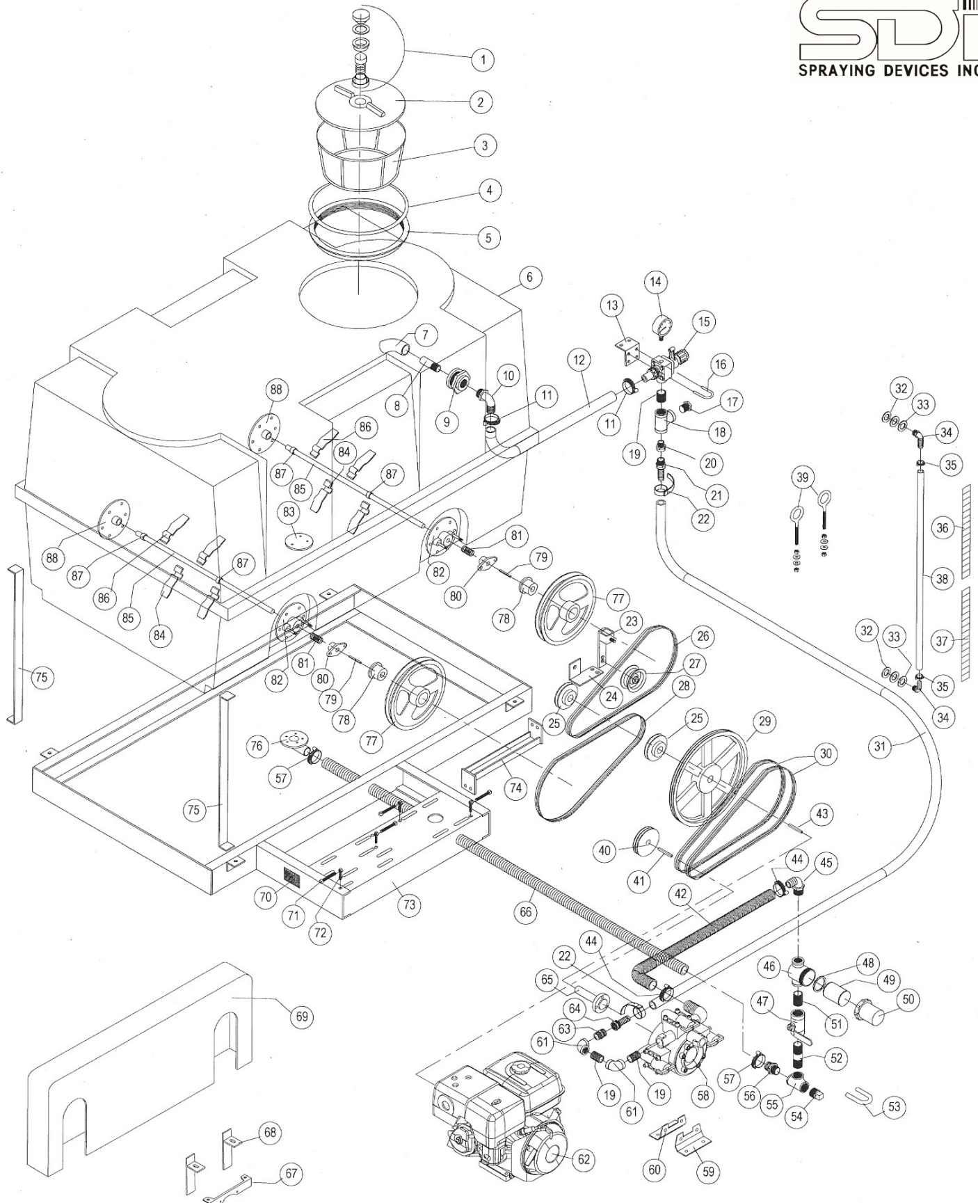
SDI Sprayer Model VM301-11HE5M
