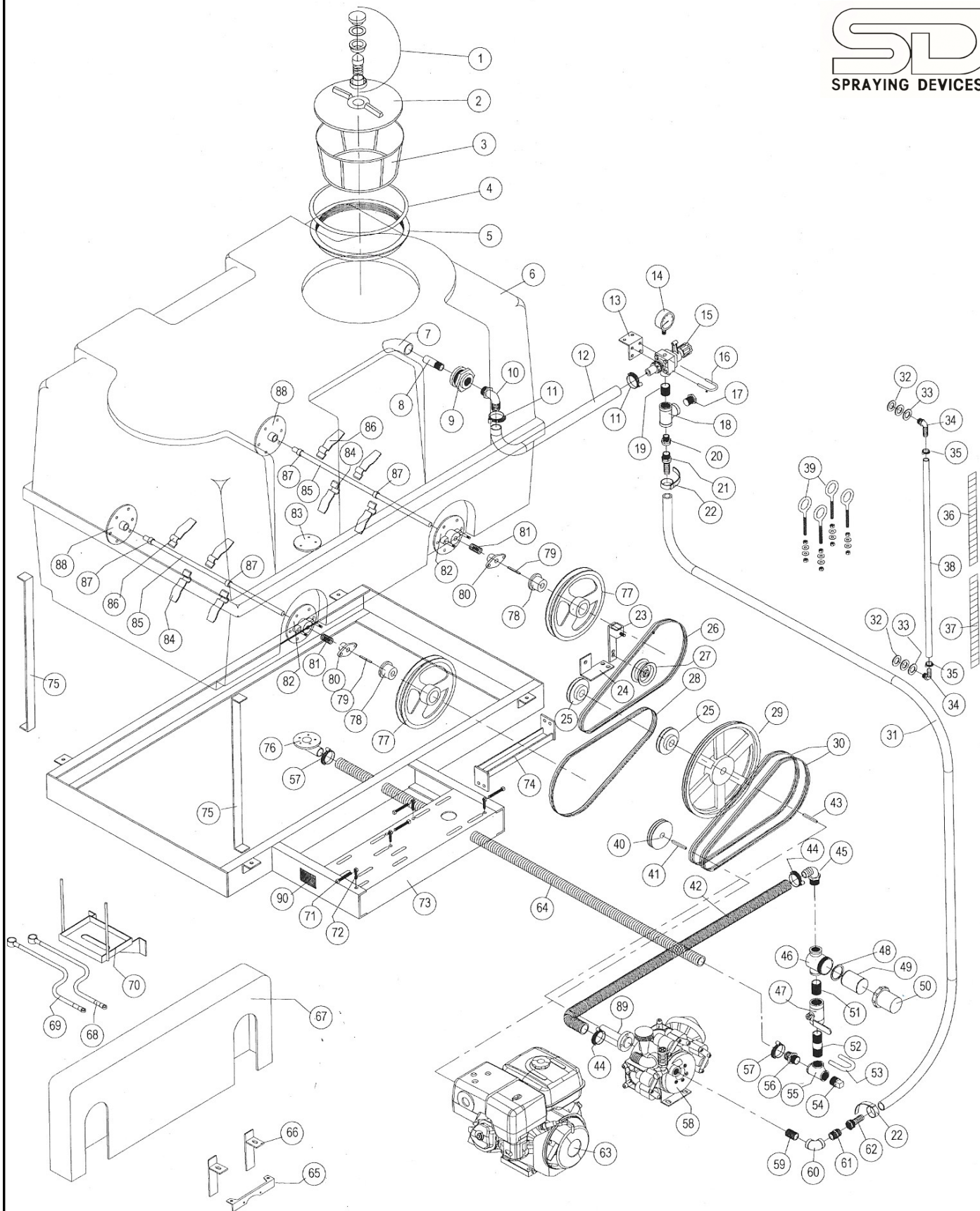
SDI Sprayer Model VM301-20HE9M
